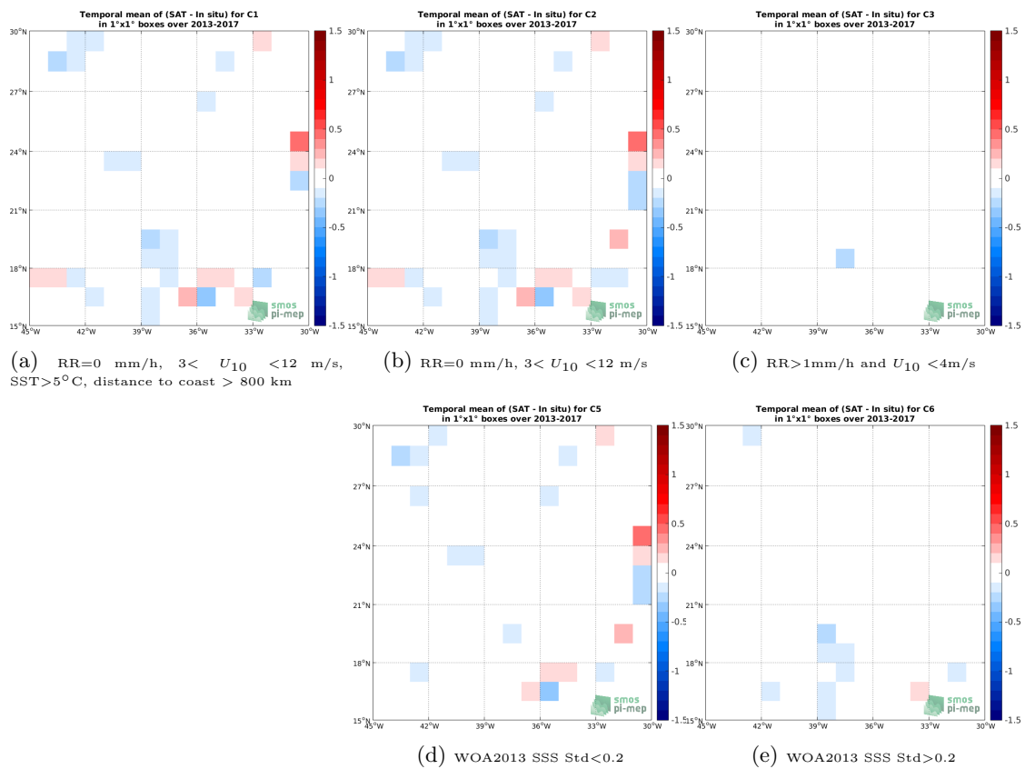
Figure 12: Temporal mean gridded over spatial boxes of size 1^\circ \times 1^\circ of \Delta\text{SSS} (SMAP SSS L4 OI v1 - Monthly (IPRC) - TSG (GOSUD-Sailing-ship)) for 5 different subdatasets corresponding to:RR=0 mm/h, 3 < U_{10} < 12 m/s, SST>5°C, distance to coast > 800 km (a), RR=0 mm/h, 3 < U_{10} < 12 m/s (b), RR>1mm/h and U_{10} < 4 m/s (c), WOA2013 SSS Std<0.2 (d), WOA2013 SSS Std>0.2 (e).
