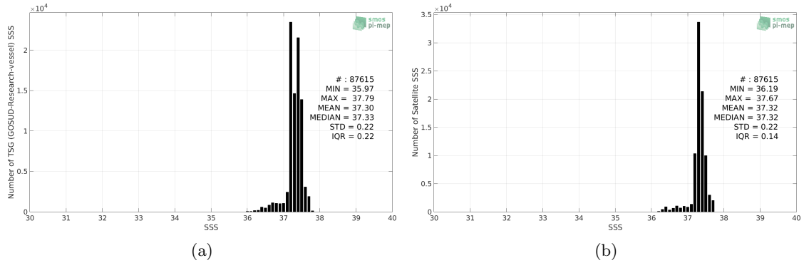
Figure 2: Histograms of SSS from TSG (GOSUD-Research-vessel) (a) and SMAP SSS L4 OI v1 - Monthly (IPRC) (b) considering all match-up pairs per bins of 0.1 over the SPURS 1 Pi-MEP region and for the full satellite product period.
