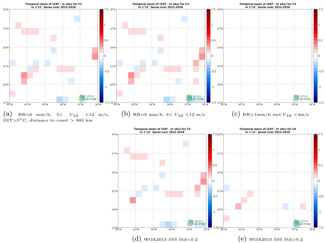
Figure 12: Temporal mean gridded over spatial boxes of size 1^\circ \times 1^\circ of \Delta\text{SSS} (SMAP SSS L4 OI v1 - Monthly (IPRC) - TSG (GOSUD-Research-vessel)) for 5 different subdatasets corresponding to:RR=0 mm/h, 3 < U_{10} < 12 m/s, SST>5°C, distance to coast > 800 km (a), RR=0 mm/h, 3 < U_{10} < 12 m/s (b), RR>1mm/h and U_{10} < 4 m/s (c), WOA2013 SSS Std<0.2 (d), WOA2013 SSS Std>0.2 (e).
