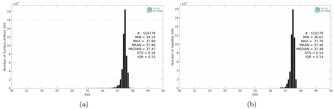
Figure 2: Histograms of SSS from Surface drifters (a) and SMAP SSS L4 OI v1 - Monthly (IPRC) (b) considering all match-up pairs per bins of 0.1 over the SPURS 1 Pi-MEP region and for the full satellite product period.
