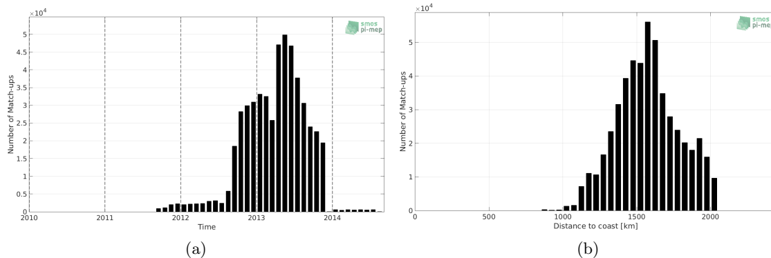
Figure 1: Number of match-ups between Surface drifters and SMAP SSS L4 OI v1 - Monthly (IPRC) SSS as a function of time (a) and as function of the distance to coast (b) over the SPURS 1 Pi-MEP region and for the full satellite product period.
