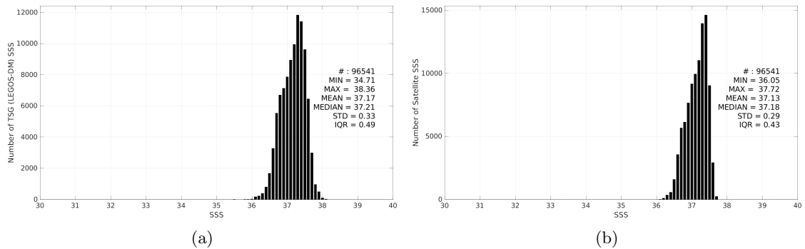
Figure 3: Histograms of SSS from TSG (LEGOS-DM) (a) and SMAP SSS L4 OI v3 - Monthly (ESR) (b) considering all match-up pairs per bins of 0.1 over the SPURS 1 Pi-MEP region and for the full satellite product period.
