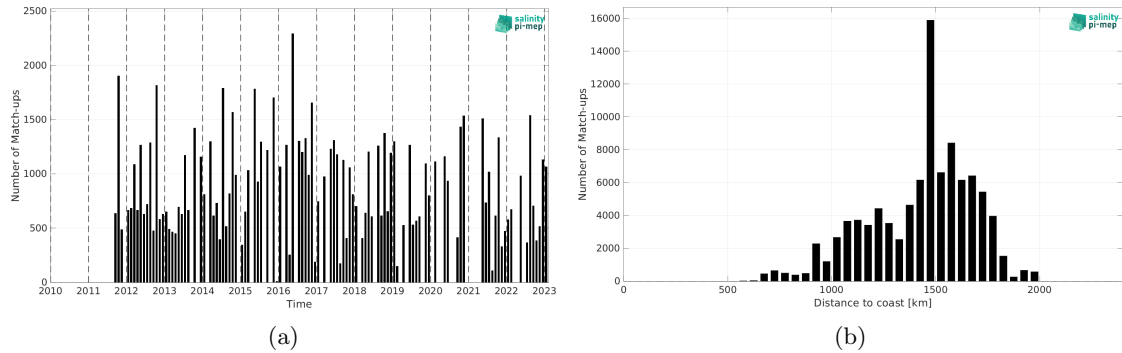
Figure 2: Number of match-ups between TSG (LEGOS-DM) and SMAP SSS L4 OI v3 - Monthly (ESR) SSS as a function of time (a) and as function of the distance to coast (b) over the SPURS 1 Pi-MEP region and for the full satellite product period.
