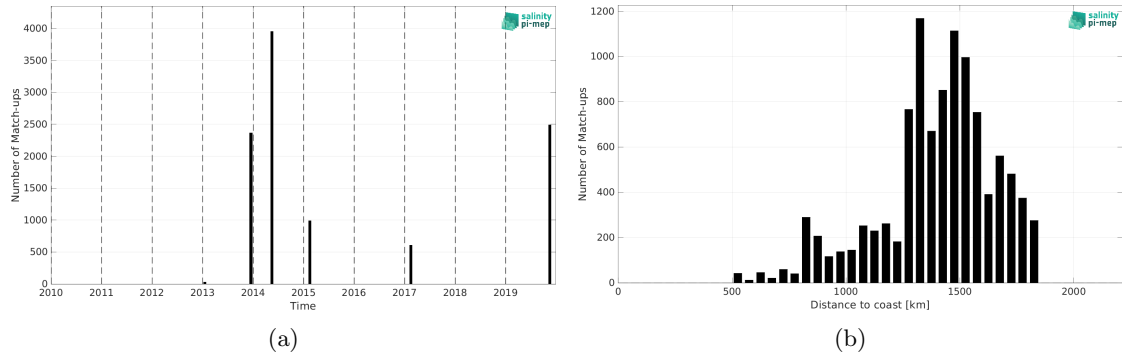
Figure 2: Number of match-ups between TSG (GOSUD-Sailing-ship) and SMAP SSS L4 OI v3 - Monthly (ESR) SSS as a function of time (a) and as function of the distance to coast (b) over the SPURS 1 Pi-MEP region and for the full satellite product period.
