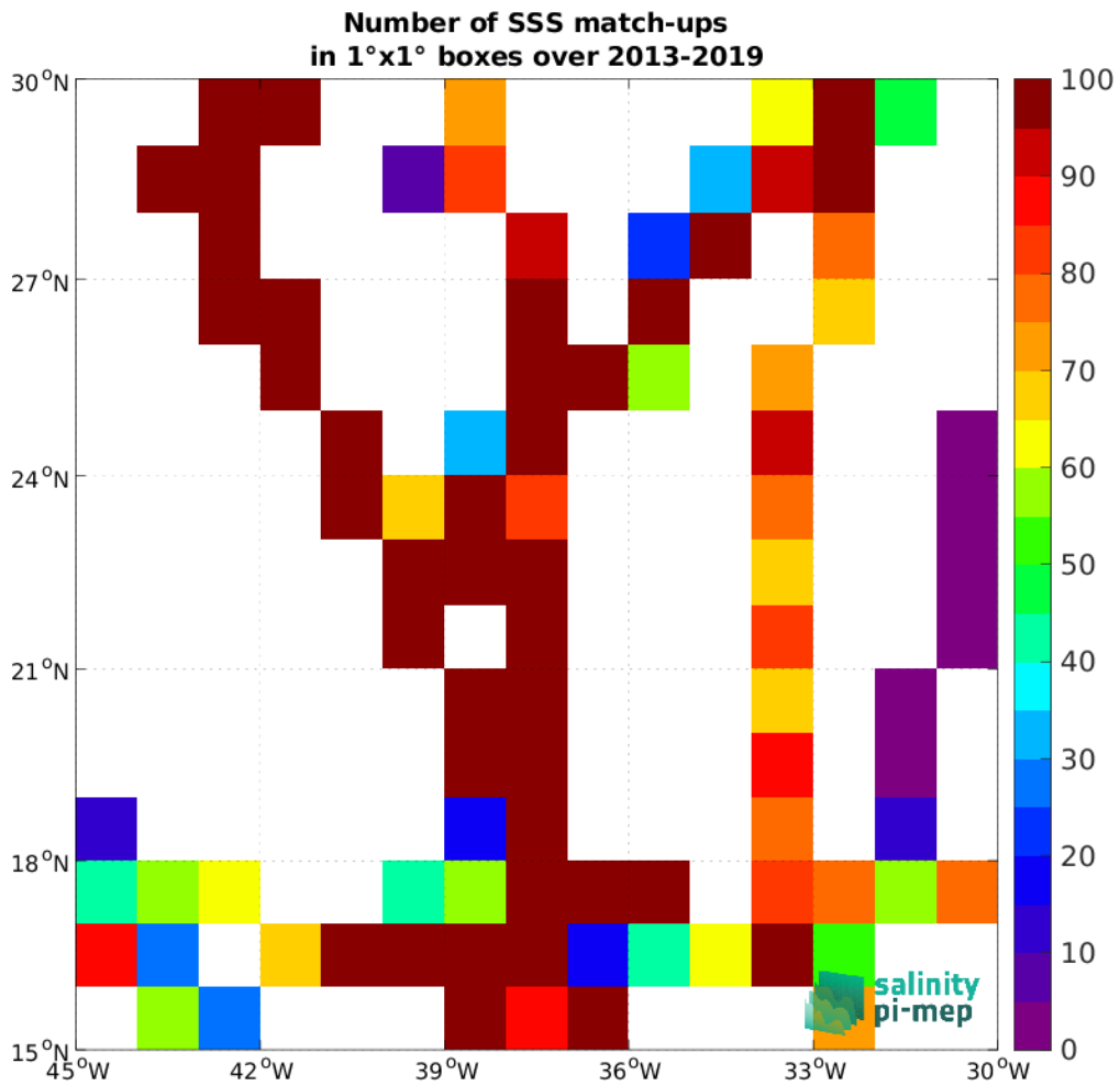
Figure 5: Number of SSS match-ups between TSG (GOSUD-Sailing-ship) SSS and the SMAP SSS L4 OI v3 - Monthly (ESR) SSS product for the SPURS 1 Pi-MEP region over 1°x1° boxes and for the full satellite product period.
