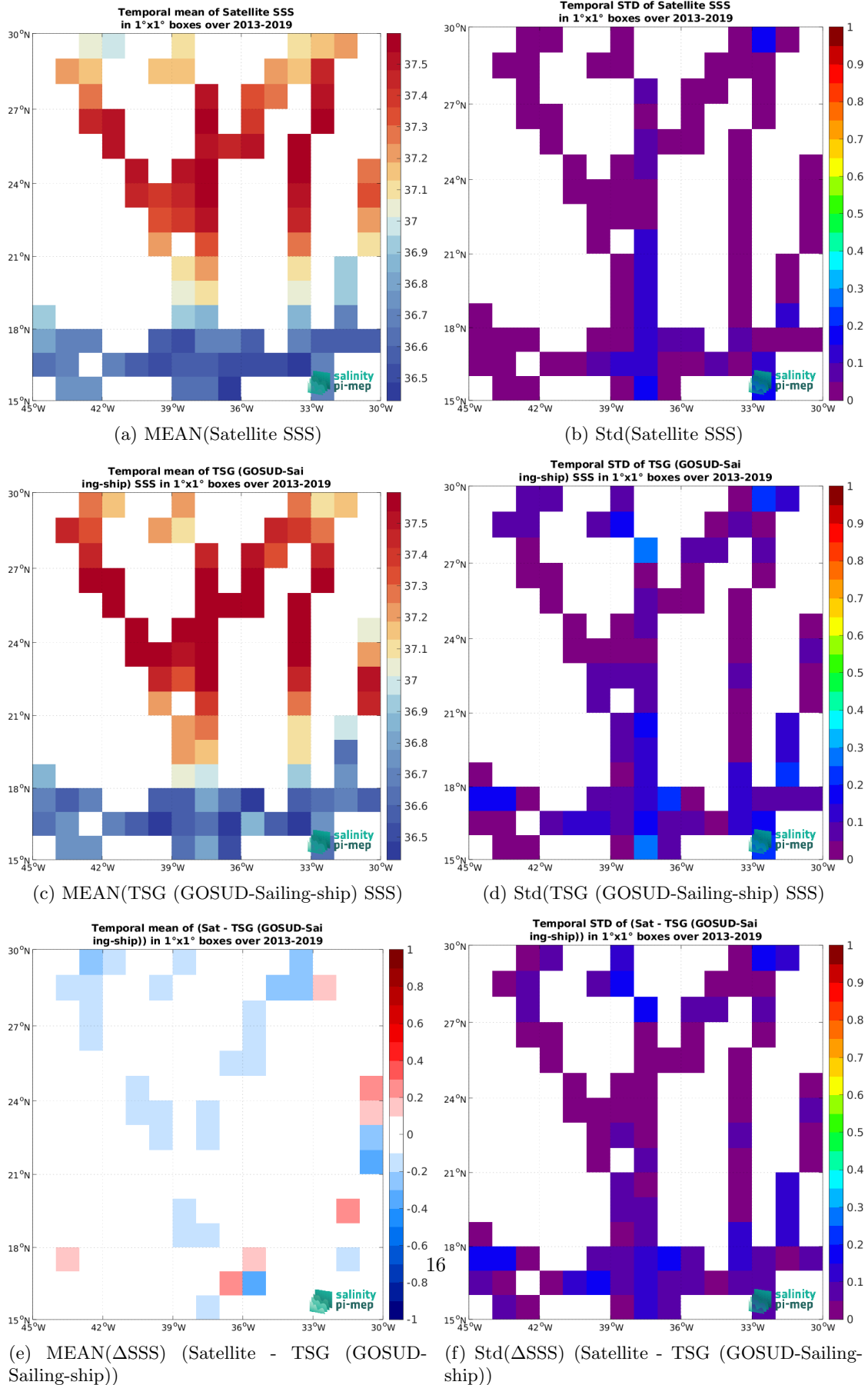
Figure 7: Temporal mean (left) and Std (right) of SSS from SMAP SSS L4 OI v3 - Monthly (ESR) (top), TSG (GOSUD-Sailing-ship) (middle), and of \Delta SSS (Satellite - TSG (GOSUD-Sailing-ship)). Only match-up pairs are used to generate these maps.
