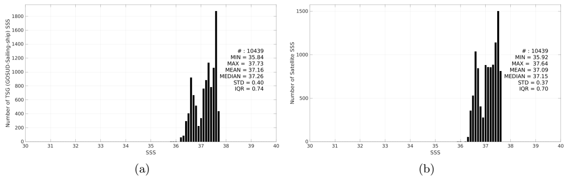
Figure 3: Histograms of SSS from TSG (GOSUD-Sailing-ship) (a) and SMAP SSS L4 OI v3 - Monthly (ESR) (b) considering all match-up pairs per bins of 0.1 over the SPURS 1 Pi-MEP region and for the full satellite product period.
