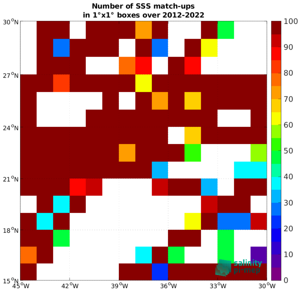
Figure 5: Number of SSS match-ups between TSG (GOSUD-Research-vessel) SSS and the SMAP SSS L4 OI v3 - Monthly (ESR) SSS product for the SPURS 1 Pi-MEP region over 1^\circ \times 1^\circ boxes and for the full satellite product period.
