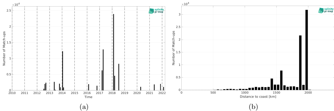
Figure 2: Number of match-ups between TSG (GOSUD-Research-vessel) and SMAP SSS L4 OI v3 - Monthly (ESR) SSS as a function of time (a) and as function of the distance to coast (b) over the SPURS 1 Pi-MEP region and for the full satellite product period.
