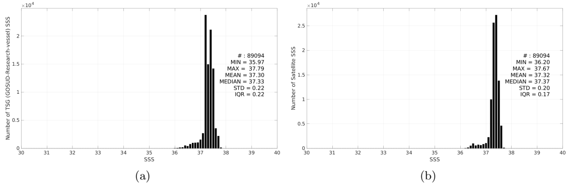
Figure 3: Histograms of SSS from TSG (GOSUD-Research-vessel) (a) and SMAP SSS L4 OI v3 - Monthly (ESR) (b) considering all match-up pairs per bins of 0.1 over the SPURS 1 Pi-MEP region and for the full satellite product period.
