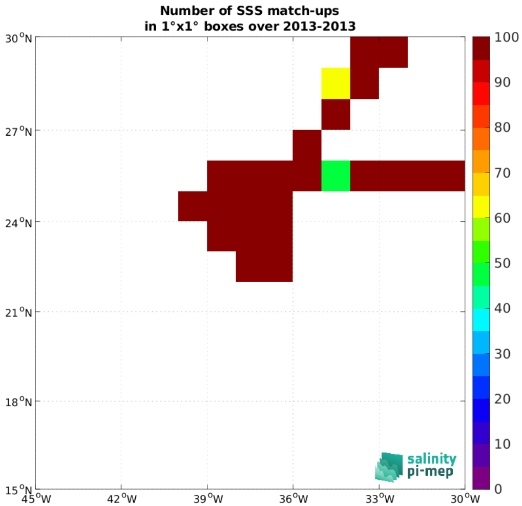
Figure 5: Number of SSS match-ups between TSG (CSIC-UTM) SSS and the SMAP SSS L4 OI v3 - Monthly (ESR) SSS product for the SPURS 1 Pi-MEP region over 1°×1° boxes and for the full satellite product period.
