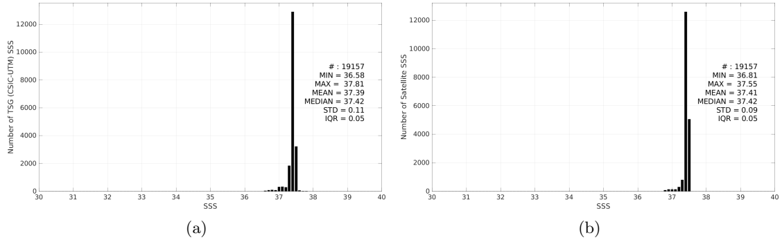
Figure 3: Histograms of SSS from TSG (CSIC-UTM) (a) and SMAP SSS L4 OI v3 - Monthly (ESR) (b) considering all match-up pairs per bins of 0.1 over the SPURS 1 Pi-MEP region and for the full satellite product period.
