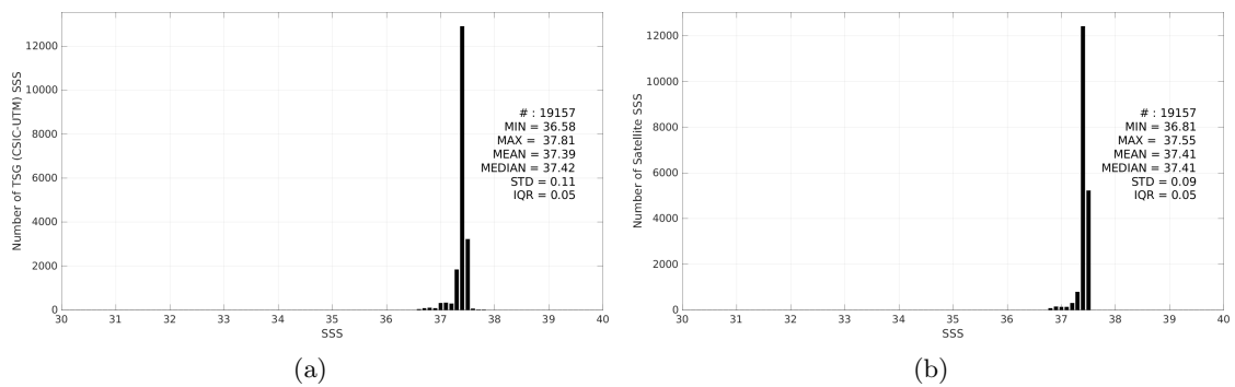
Figure 3: Histograms of SSS from TSG (CSIC-UTM) (a) and SMAP SSS L4 OI v3 - Monthly (ESR) (b) considering all match-up pairs per bins of 0.1 over the SPURS 1 Pi-MEP region and for the full satellite product period.
