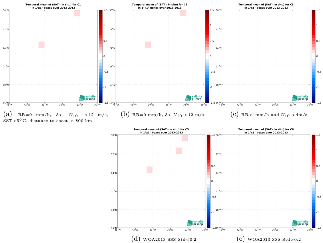
Figure 14: Temporal mean gridded over spatial boxes of size 1^\circ \times 1^\circ of \Delta SSS (SMAP SSS L4 OI v3 - Monthly (ESR) - TSG (CSIC-UTM)) for 5 different subdatasets corresponding to: RR=0 mm/h, 3 < U_{10} < 12 m/s, SST > 5^\circ C , distance to coast > 800 km (a), RR=0 mm/h, 3 < U_{10} < 12 m/s (b), RR > 1 mm/h and U_{10} < 4 m/s (c), WOA2013 SSS Std < 0.2 (d), WOA2013 SSS Std > 0.2 (e).
