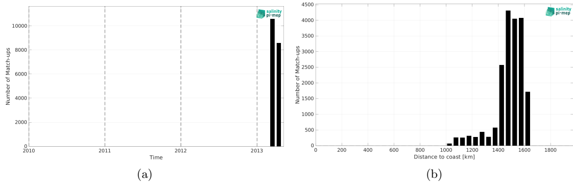
Figure 2: Number of match-ups between TSG (CSIC-UTM) and SMAP SSS L4 OI v3 - Monthly (ESR) SSS as a function of time (a) and as function of the distance to coast (b) over the SPURS 1 Pi-MEP region and for the full satellite product period.
