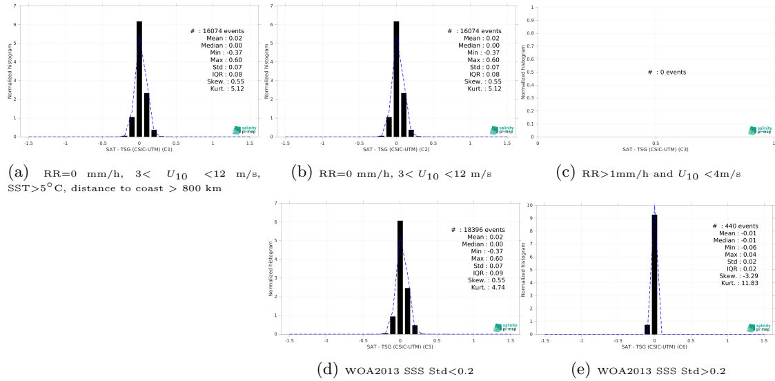
Figure 15: Normalized histogram of \Delta\text{SSS} (SMAP SSS L4 OI v3 - Monthly (ESR) - TSG (CSIC-UTM)) for 5 different subdatasets corresponding to: RR=0 mm/h, 3 < U_{10} < 12 m/s, SST > 5^{\circ}\text{C} , distance to coast > 800 km (a), RR=0 mm/h, 3 < U_{10} < 12 m/s (b), RR > 1\text{mm/h} and U_{10} < 4\text{m/s} (c), WOA2013 SSS Std < 0.2 (d), WOA2013 SSS Std > 0.2 (e).
