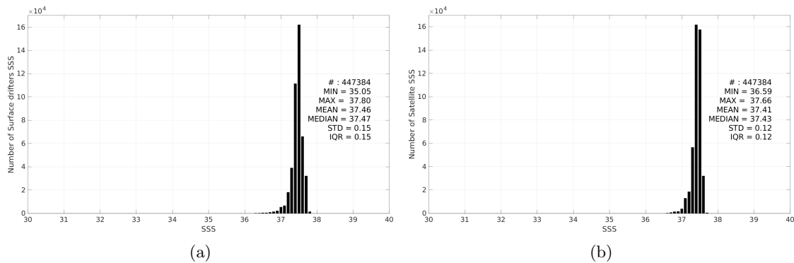
Figure 3: Histograms of SSS from Surface drifters (a) and SMAP SSS L4 OI v3 - Monthly (ESR) (b) considering all match-up pairs per bins of 0.1 over the SPURS 1 Pi-MEP region and for the full satellite product period.
