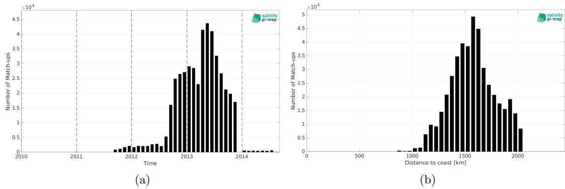
Figure 2: Number of match-ups between Surface drifters and SMAP SSS L4 OI v3 - Monthly (ESR) SSS as a function of time (a) and as function of the distance to coast (b) over the SPURS 1 Pi-MEP region and for the full satellite product period.
