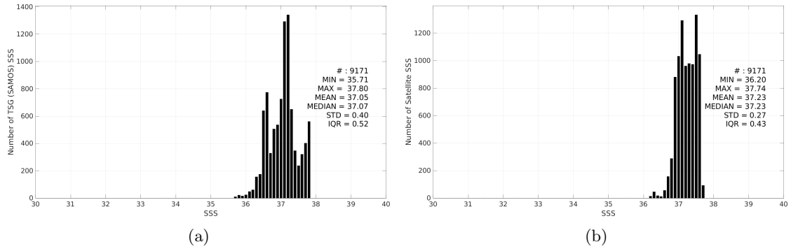
Figure 3: Histograms of SSS from TSG (SAMOS) (a) and SMAP SSS L4 OI v3 - Daily (ESR) (b) considering all match-up pairs per bins of 0.1 over the SPURS 1 Pi-MEP region and for the full satellite product period.
