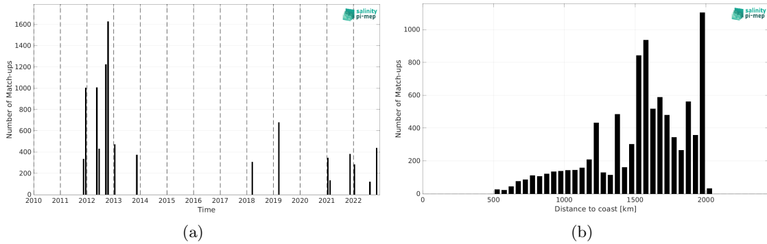
Figure 2: Number of match-ups between TSG (SAMOS) and SMAP SSS L4 OI v3 - Daily (ESR) SSS as a function of time (a) and as function of the distance to coast (b) over the SPURS 1 Pi-MEP region and for the full satellite product period.
