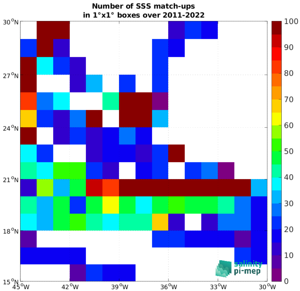
Figure 5: Number of SSS match-ups between TSG (SAMOS) SSS and the SMAP SSS L4 OI v3 - Daily (ESR) SSS product for the SPURS 1 Pi-MEP region over 1°x1° boxes and for the full satellite product period.
