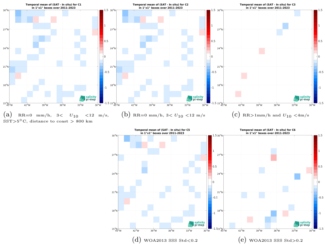
Figure 14: Temporal mean gridded over spatial boxes of size 1^\circ \times 1^\circ of \Delta SSS (SMAP SSS L4 OI v3 - Daily (ESR) - TSG (LEGOS-DM)) for 5 different subdatasets corresponding to: RR=0 mm/h, 3 < U_{10} < 12 m/s, SST > 5^\circ C , distance to coast > 800 km (a), RR=0 mm/h, 3 < U_{10} < 12 m/s (b), RR > 1 mm/h and U_{10} < 4 m/s (c), WOA2013 SSS Std < 0.2 (d), WOA2013 SSS Std > 0.2 (e).
