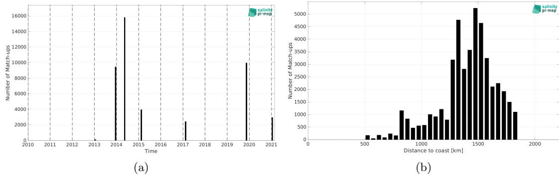
Figure 2: Number of match-ups between TSG (GOSUD-Sailing-ship) and SMAP SSS L4 OI v3 - Daily (ESR) SSS as a function of time (a) and as function of the distance to coast (b) over the SPURS 1 Pi-MEP region and for the full satellite product period.
