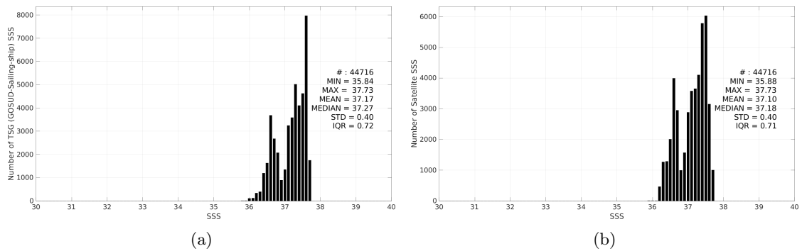
Figure 3: Histograms of SSS from TSG (GOSUD-Sailing-ship) (a) and SMAP SSS L4 OI v3 - Daily (ESR) (b) considering all match-up pairs per bins of 0.1 over the SPURS 1 Pi-MEP region and for the full satellite product period.
