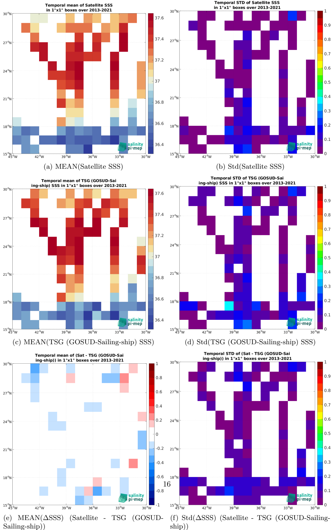
Figure 7: Temporal mean (left) and Std (right) of SSS from SMAP SSS L4 OI v3 - Daily (ESR) (top), TSG (GOSUD-Sailing-ship) (middle), and of \Delta SSS (Satellite - TSG (GOSUD-Sailing-ship)). Only match-up pairs are used to generate these maps.
