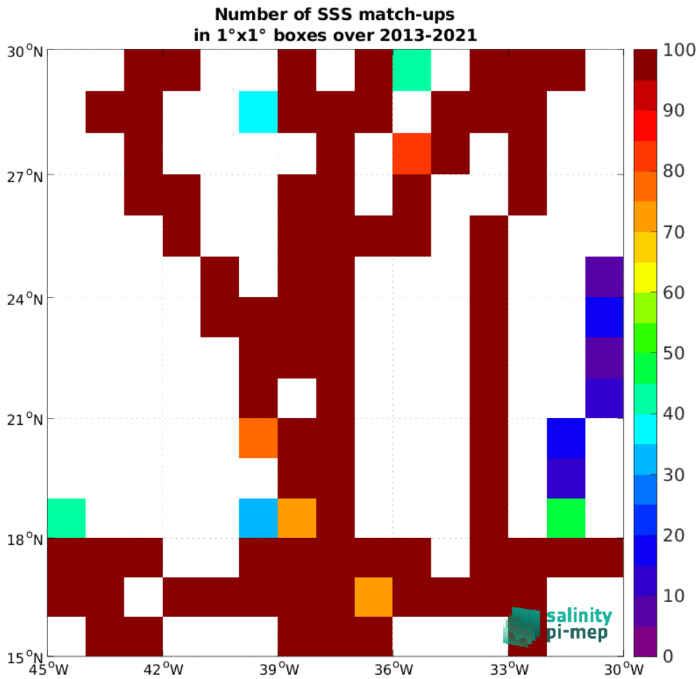
Figure 5: Number of SSS match-ups between TSG (GOSUD-Sailing-ship) SSS and the SMAP SSS L4 OI v3 - Daily (ESR) SSS product for the SPURS 1 Pi-MEP region over 1^\circ \times 1^\circ boxes and for the full satellite product period.
