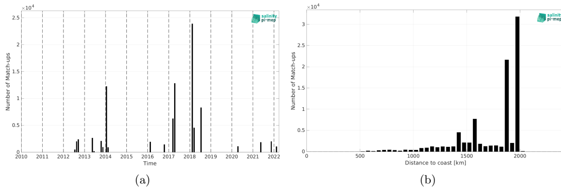
Figure 2: Number of match-ups between TSG (GOSUD-Research-vessel) and SMAP SSS L4 OI v3 - Daily (ESR) SSS as a function of time (a) and as function of the distance to coast (b) over the SPURS 1 Pi-MEP region and for the full satellite product period.
