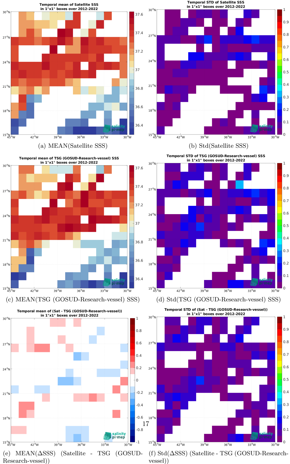
Figure 7: Temporal mean (left) and Std (right) of SSS from SMAP SSS L4 OI v3 - Daily (ESR) (top), TSG (GOSUD-Research-vessel) (middle), and of \Delta SSS (Satellite - TSG (GOSUD-Research-vessel)). Only match-up pairs are used to generate these maps.
