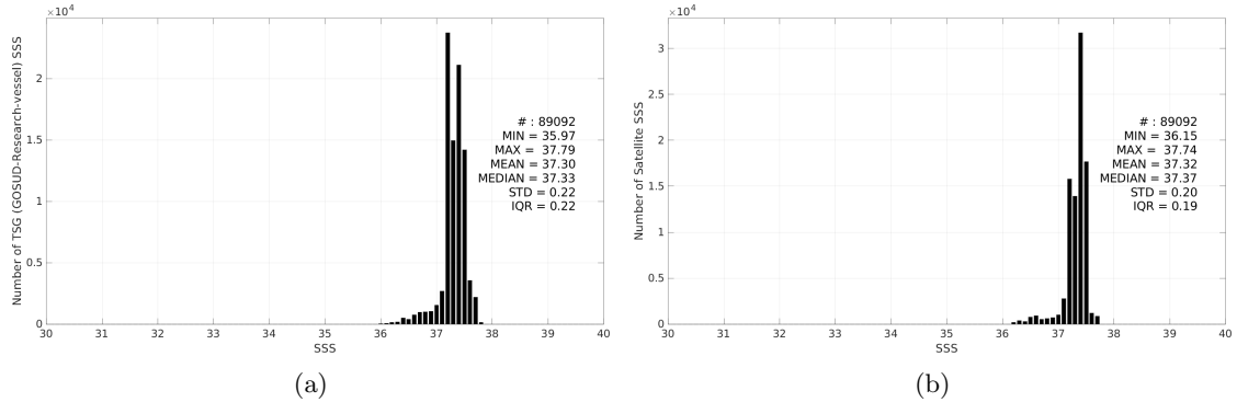
Figure 3: Histograms of SSS from TSG (GOSUD-Research-vessel) (a) and SMAP SSS L4 OI v3 - Daily (ESR) (b) considering all match-up pairs per bins of 0.1 over the SPURS 1 Pi-MEP region and for the full satellite product period.
