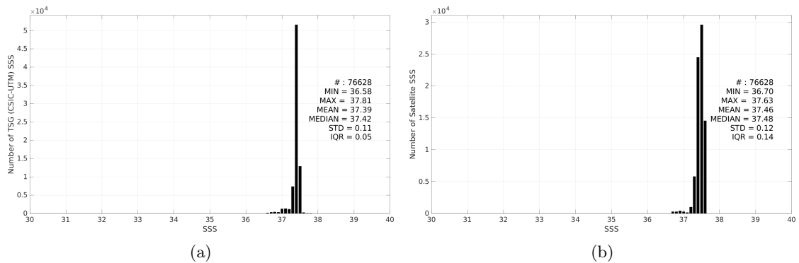
Figure 3: Histograms of SSS from TSG (CSIC-UTM) (a) and SMAP SSS L4 OI v3 - Daily (ESR) (b) considering all match-up pairs per bins of 0.1 over the SPURS 1 Pi-MEP region and for the full satellite product period.
