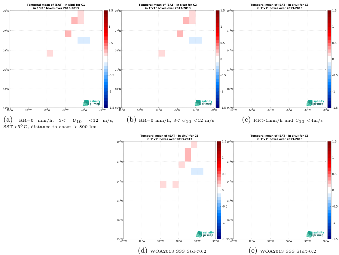
Figure 14: Temporal mean gridded over spatial boxes of size 1^\circ \times 1^\circ of \Delta SSS (SMAP SSS L4 OI v3 - Daily (ESR) - TSG (CSIC-UTM)) for 5 different subdatasets corresponding to:RR=0 mm/h, 3 < U_{10} < 12 m/s, SST >5^\circ\text{C} , distance to coast > 800 km (a), RR=0 mm/h, 3 < U_{10} < 12 m/s (b), RR >1 mm/h and U_{10} < 4 m/s (c), WOA2013 SSS Std <0.2 (d), WOA2013 SSS Std >0.2 (e).
