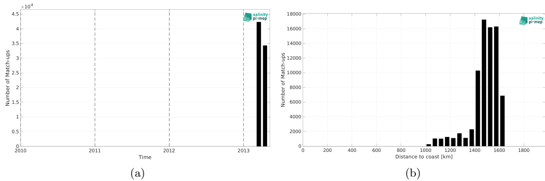
Figure 2: Number of match-ups between TSG (CSIC-UTM) and SMAP SSS L4 OI v3 - Daily (ESR) SSS as a function of time (a) and as function of the distance to coast (b) over the SPURS 1 Pi-MEP region and for the full satellite product period.
