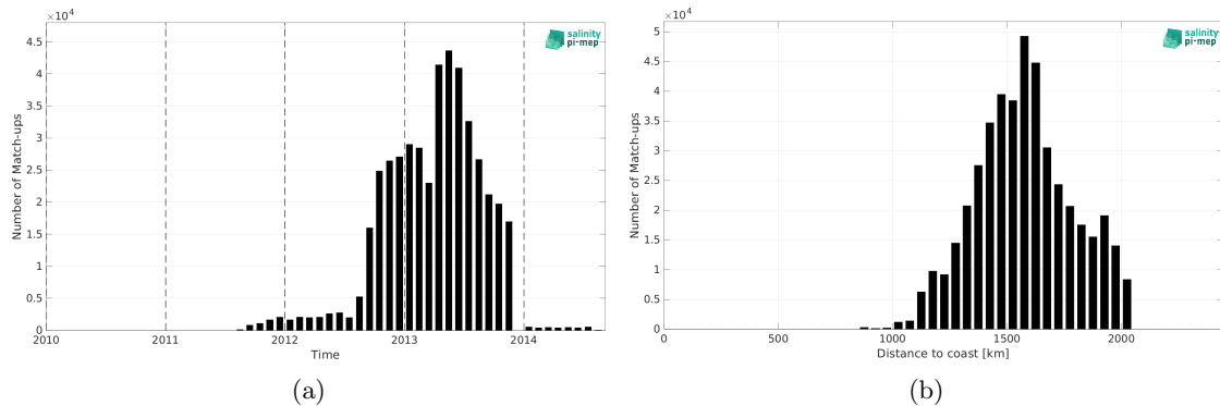
Figure 2: Number of match-ups between Surface drifters and SMAP SSS L4 OI v3 - Daily (ESR) SSS as a function of time (a) and as function of the distance to coast (b) over the SPURS 1 Pi-MEP region and for the full satellite product period.
