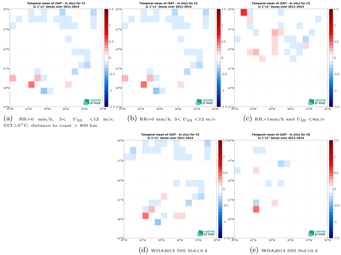
Figure 13: Temporal mean gridded over spatial boxes of size 1^\circ \times 1^\circ of \Delta SSS (SMAP SSS L4 OI v3 - Daily (ESR) - Surface drifters) for 5 different subdatasets corresponding to:RR=0 mm/h, 3 < U_{10} < 12 m/s, SST >5^\circ C, distance to coast > 800 km (a), RR=0 mm/h, 3 < U_{10} < 12 m/s (b), RR >1 mm/h and U_{10} < 4 m/s (c), WOA2013 SSS Std <0.2 (d), WOA2013 SSS Std >0.2 (e).
