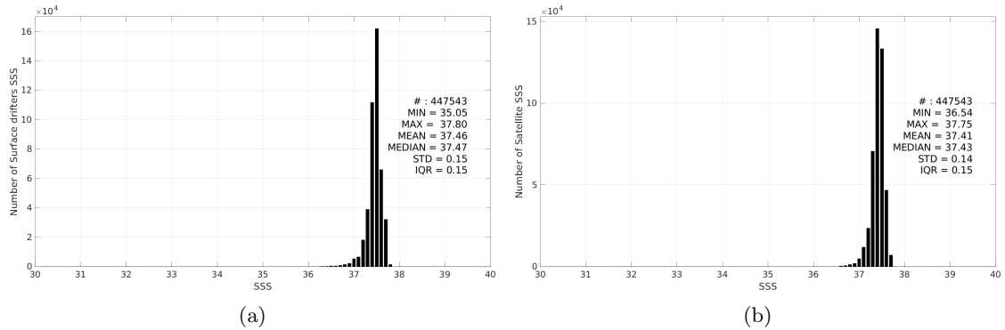
Figure 3: Histograms of SSS from Surface drifters (a) and SMAP SSS L4 OI v3 - Daily (ESR) (b) considering all match-up pairs per bins of 0.1 over the SPURS 1 Pi-MEP region and for the full satellite product period.
