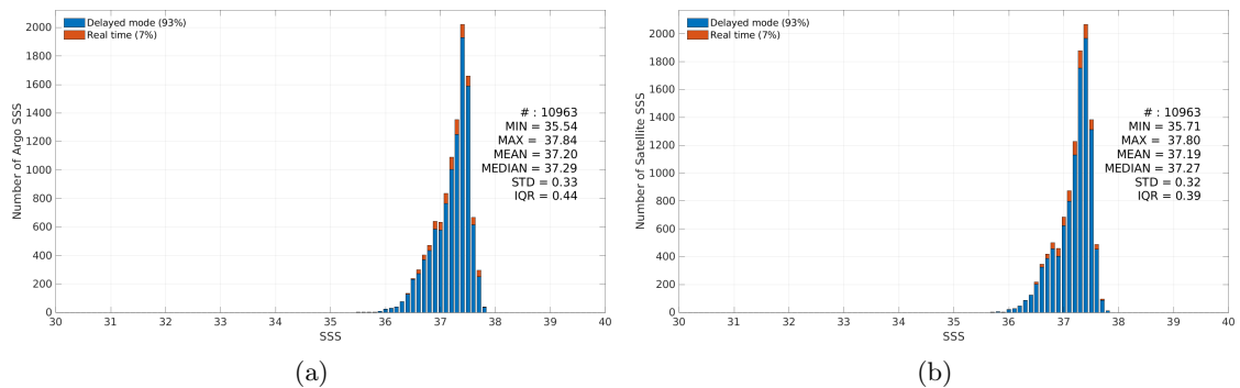
Figure 3: Histograms of SSS from Argo (a) and SMAP SSS L4 OI v3 - Daily (ESR) (b) considering all match-up pairs per bins of 0.1 over the SPURS 1 Pi-MEP region and for the full satellite product period.
