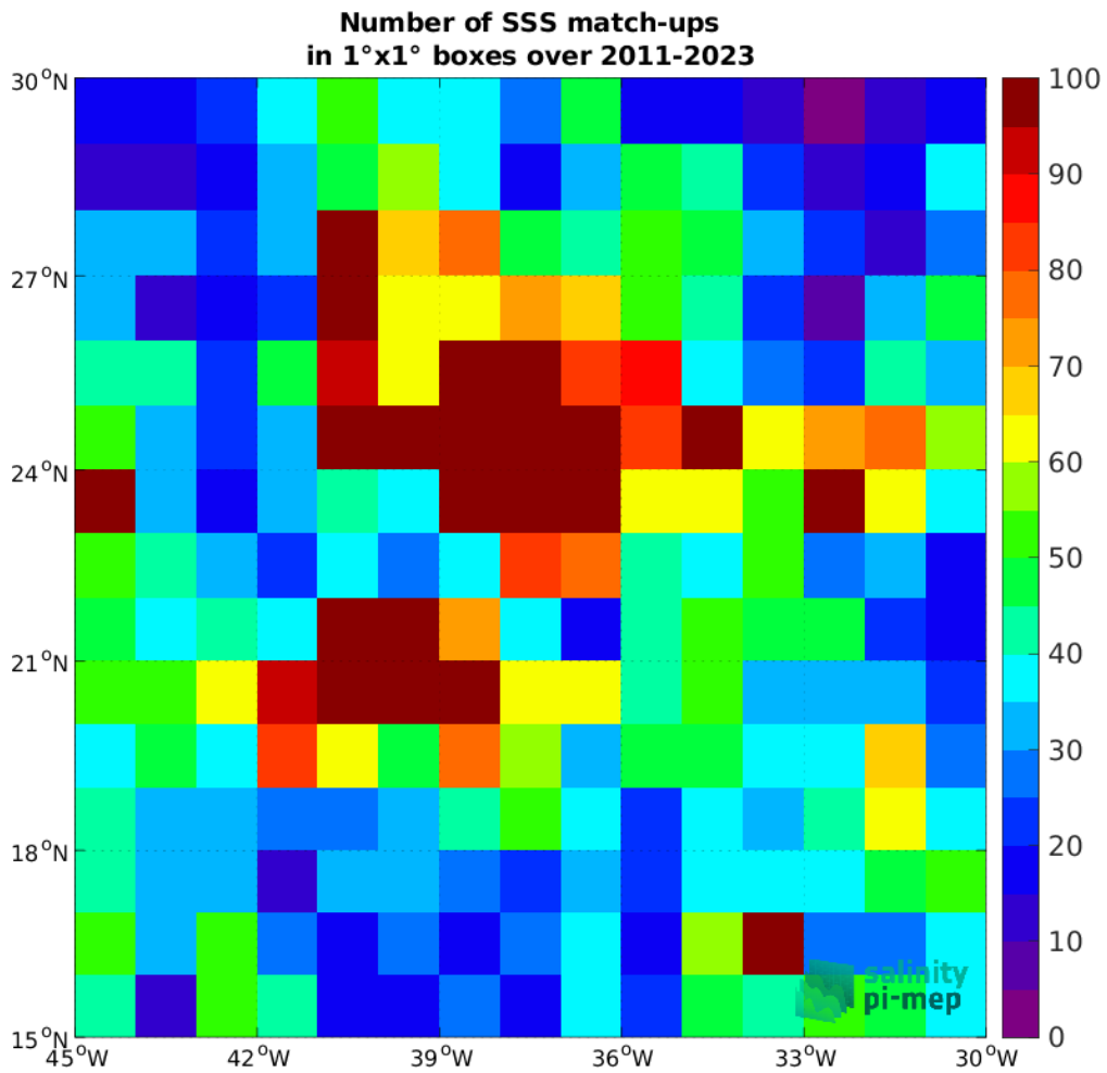
Figure 5: Number of SSS match-ups between Argo SSS and the SMAP SSS L4 OI v3 - Daily (ESR) SSS product for the SPURS 1 Pi-MEP region over 1^\circ \times 1^\circ boxes and for the full satellite product period.
