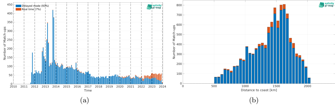
Figure 2: Number of match-ups between Argo and SMAP SSS L4 OI v3 - Daily (ESR) SSS as a function of time (a) and as function of the distance to coast (b) over the SPURS 1 Pi-MEP region and for the full satellite product period.
