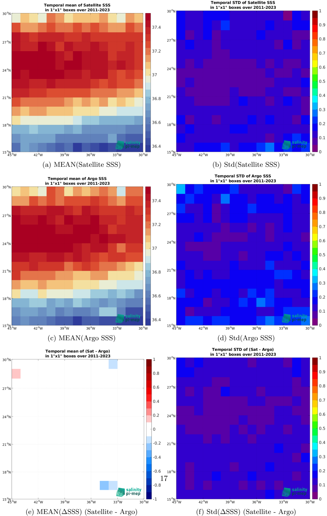
Figure 7: Temporal mean (left) and Std (right) of SSS from SMAP SSS L4 OI v3 - Daily (ESR) (top), Argo (middle), and of \Delta SSS (Satellite - Argo). Only match-up pairs are used to generate these maps.
