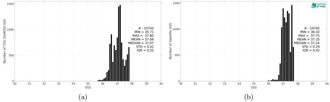
Figure 2: Histograms of SSS from TSG (SAMOS) (a) and SMAP SSS L4 OI v2 - 7 Days (ESR) (b) considering all match-up pairs per bins of 0.1 over the SPURS 1 Pi-MEP region and for the full satellite product period.
