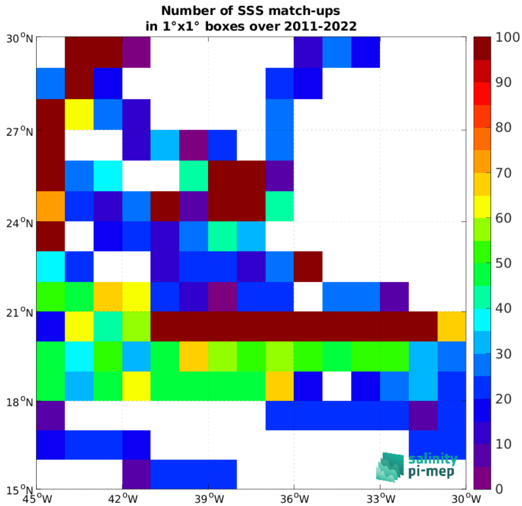
Figure 4: Number of SSS match-ups between TSG (SAMOS) SSS and the SMAP SSS L4 OI v2 - 7 Days (ESR) SSS product for the SPURS 1 Pi-MEP region over 1°x1° boxes and for the full satellite product period.
