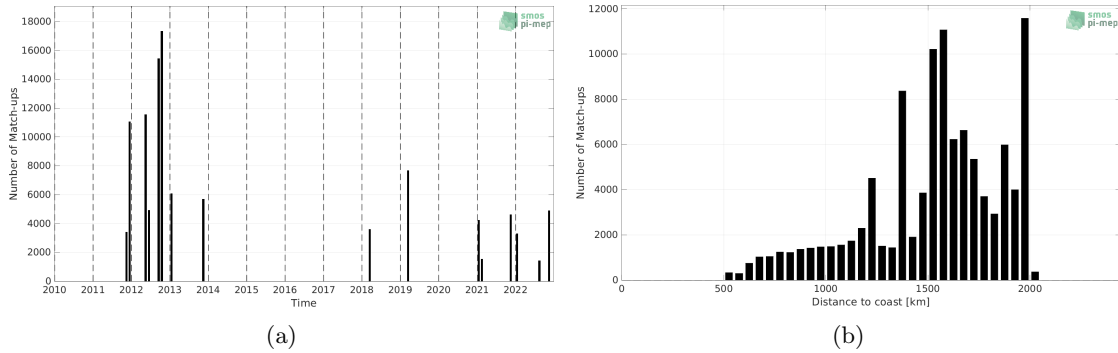
Figure 1: Number of match-ups between TSG (SAMOS) and SMAP SSS L4 OI v2 - 7 Days (ESR) SSS as a function of time (a) and as function of the distance to coast (b) over the SPURS 1 Pi-MEP region and for the full satellite product period.
