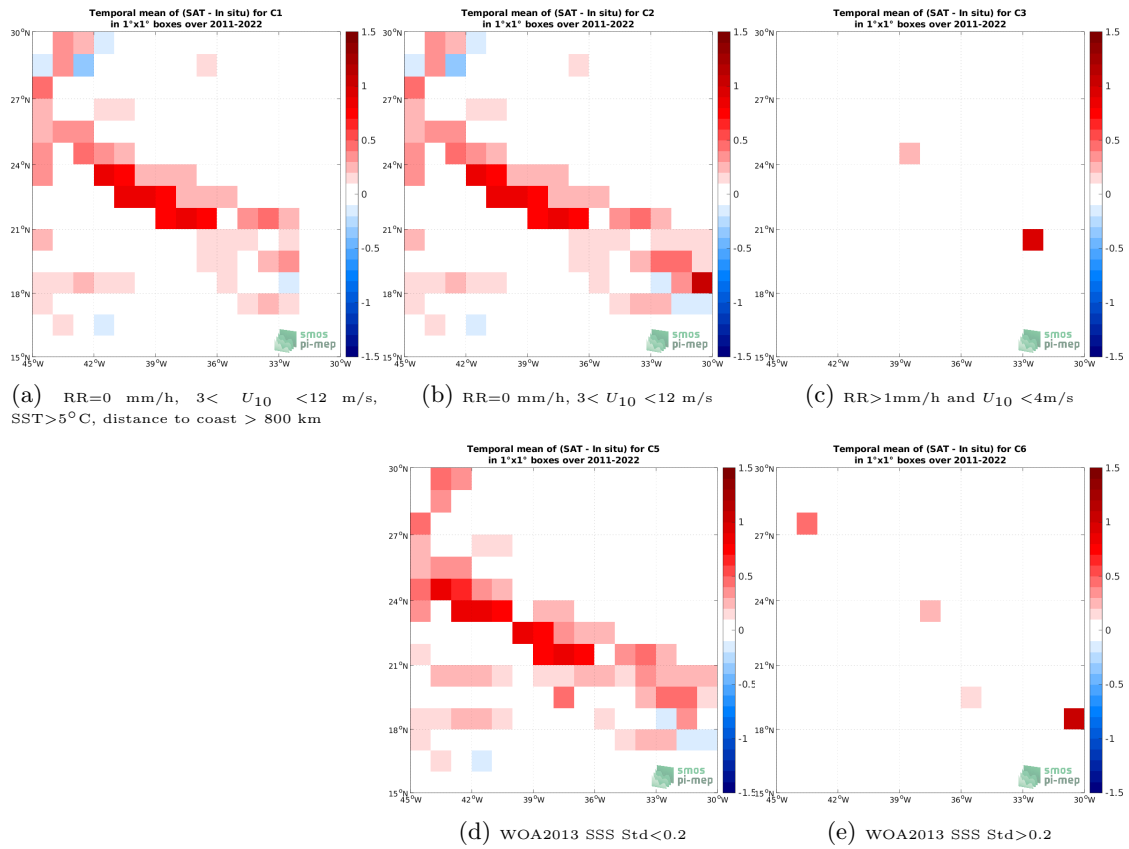
Figure 12: Temporal mean gridded over spatial boxes of size 1^\circ \times 1^\circ of \Delta SSS (SMAP SSS L4 OI v2 - 7 Days (ESR) - TSG (SAMOS)) for 5 different subdatasets corresponding to:RR=0 mm/h, 3 < U_{10} < 12 m/s, SST >5^\circ C, distance to coast > 800 km (a), RR=0 mm/h, 3 < U_{10} < 12 m/s (b), RR >1 mm/h and U_{10} < 4 m/s (c), WOA2013 SSS Std <0.2 (d), WOA2013 SSS Std >0.2 (e).
