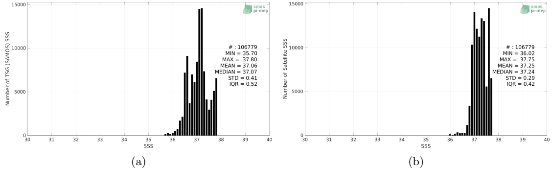
Figure 2: Histograms of SSS from TSG (SAMOS) (a) and SMAP SSS L4 OI v2 - 7 Days (ESR) (b) considering all match-up pairs per bins of 0.1 over the SPURS 1 Pi-MEP region and for the full satellite product period.
