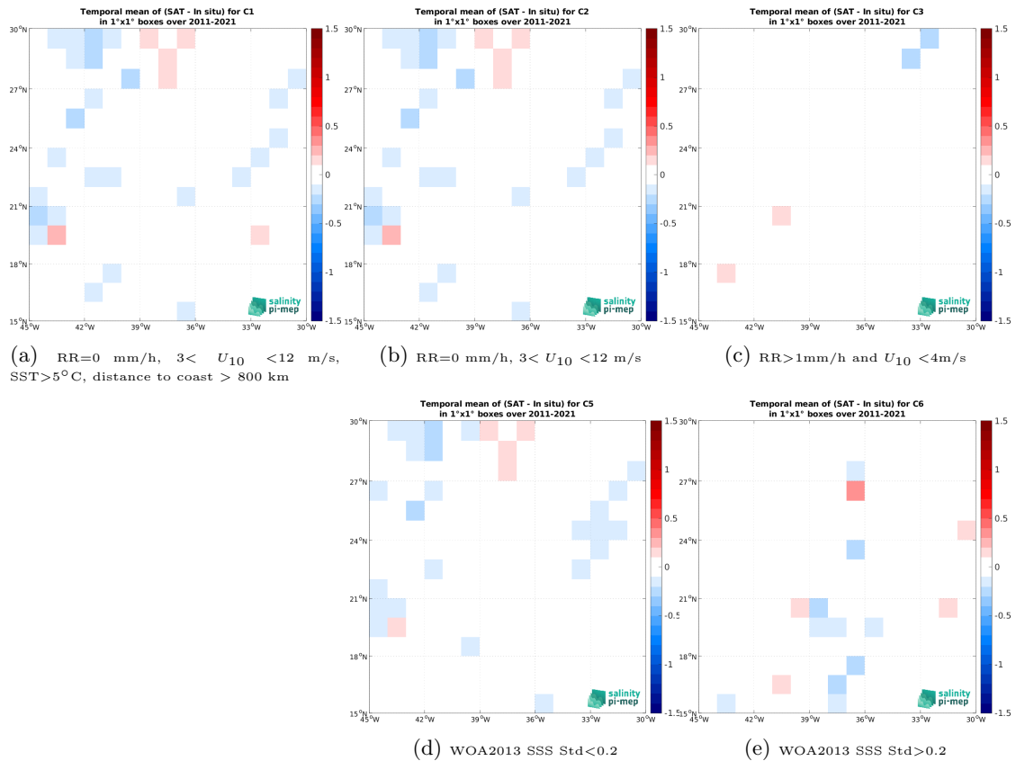
Figure 12: Temporal mean gridded over spatial boxes of size 1^\circ \times 1^\circ of \Delta SSS (SMAP SSS L4 OI v2 - 7 Days (ESR) - TSG (LEGOS-DM)) for 5 different subdatasets corresponding to: RR=0 mm/h, 3 < U_{10} < 12 m/s, SST > 5^\circ C , distance to coast > 800 km (a), RR=0 mm/h, 3 < U_{10} < 12 m/s (b), RR > 1 mm/h and U_{10} < 4 m/s (c), WOA2013 SSS Std <0.2 (d), WOA2013 SSS Std >0.2 (e).
