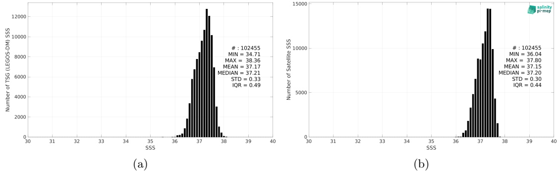
Figure 2: Histograms of SSS from TSG (LEGOS-DM) (a) and SMAP SSS L4 OI v2 - 7 Days (ESR) (b) considering all match-up pairs per bins of 0.1 over the SPURS 1 Pi-MEP region and for the full satellite product period.
