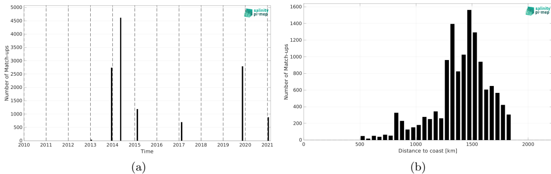
Figure 1: Number of match-ups between TSG (GOSUD-Sailing-ship) and SMAP SSS L4 OI v2 - 7 Days (ESR) SSS as a function of time (a) and as function of the distance to coast (b) over the SPURS 1 Pi-MEP region and for the full satellite product period.
