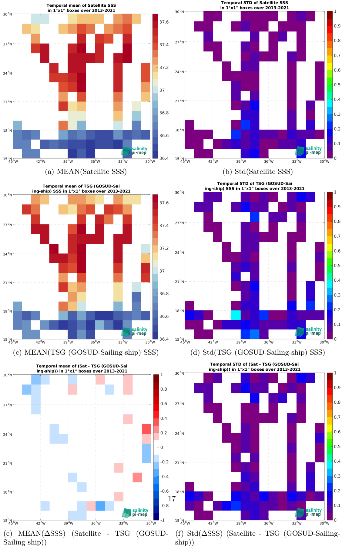
Figure 6: Temporal mean (left) and Std (right) of SSS from SMAP SSS L4 OI v2 - 7 Days (ESR) (top), TSG (GOSUD-Sailing-ship) (middle), and of \Delta SSS (Satellite - TSG (GOSUD-Sailing-ship)). Only match-up pairs are used to generate these maps.
