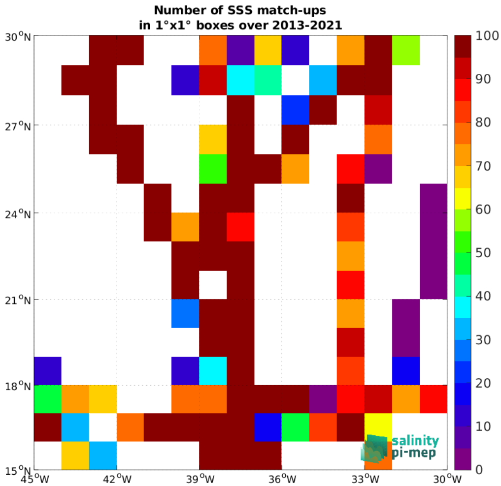
Figure 4: Number of SSS match-ups between TSG (GOSUD-Sailing-ship) SSS and the SMAP SSS L4 OI v2 - 7 Days (ESR) SSS product for the SPURS 1 Pi-MEP region over 1°x1° boxes and for the full satellite product period.
