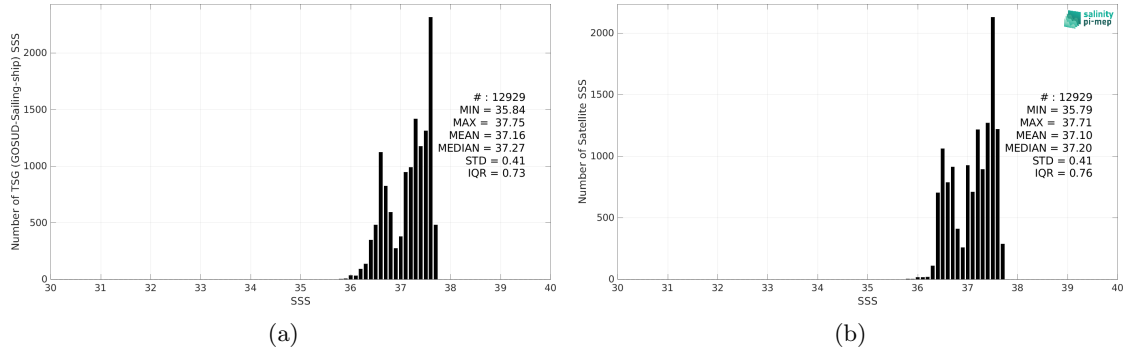
Figure 2: Histograms of SSS from TSG (GOSUD-Sailing-ship) (a) and SMAP SSS L4 OI v2 - 7 Days (ESR) (b) considering all match-up pairs per bins of 0.1 over the SPURS 1 Pi-MEP region and for the full satellite product period.
