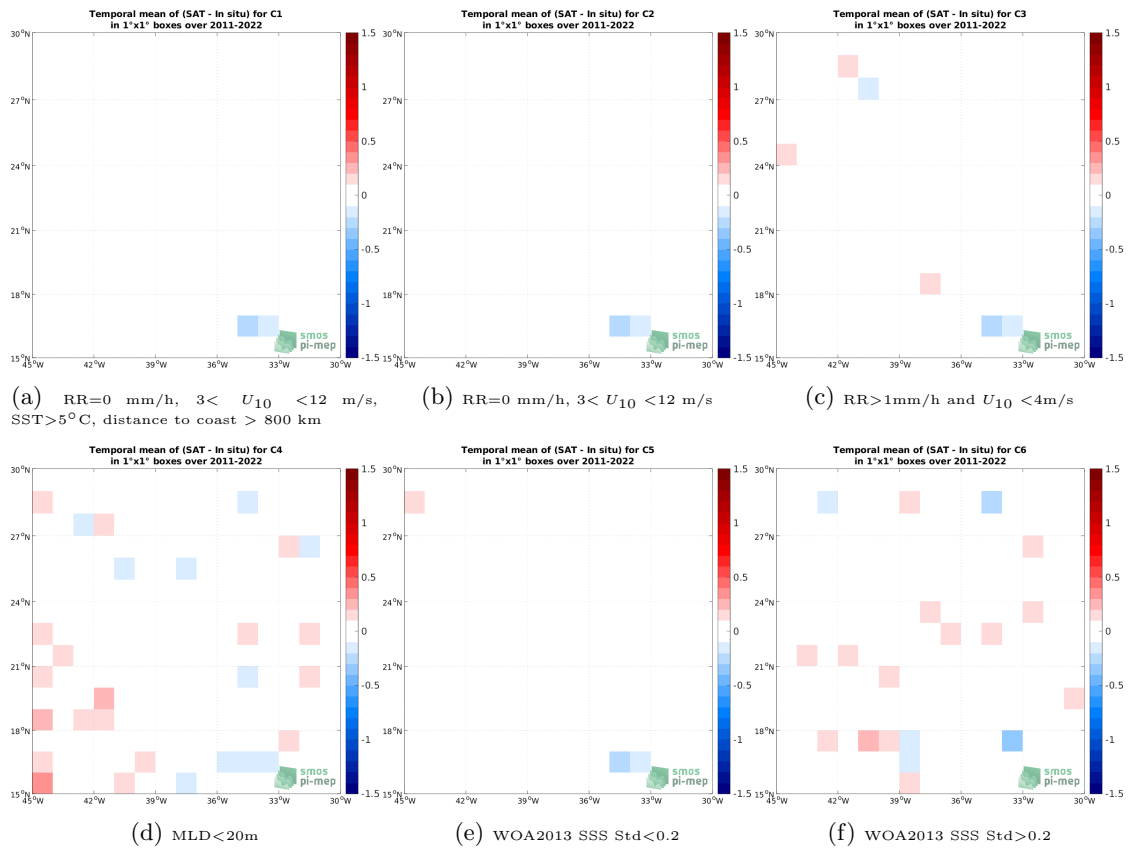
Figure 12: Temporal mean gridded over spatial boxes of size 1^\circ \times 1^\circ of \Delta SSS (SMAP SSS L4 OI v2 - 7 Days (ESR) - Argo) for 6 different subdatasets corresponding to:RR=0 mm/h, 3 < U_{10} < 12 m/s, SST >5^\circ C, distance to coast > 800 km (a), RR=0 mm/h, 3 < U_{10} < 12 m/s (b), RR >1 mm/h and U_{10} < 4 m/s (c),MLD <20 m (d),WOA2013 SSS Std <0.2 (e),WOA2013 SSS Std >0.2 (f).
