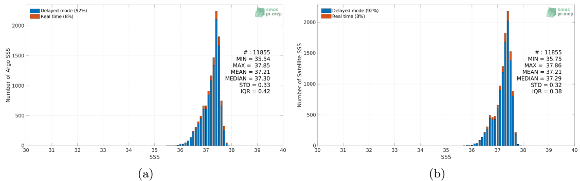
Figure 2: Histograms of SSS from Argo (a) and SMAP SSS L4 OI v2 - 7 Days (ESR) (b) considering all match-up pairs per bins of 0.1 over the SPURS 1 Pi-MEP region and for the full satellite product period.
