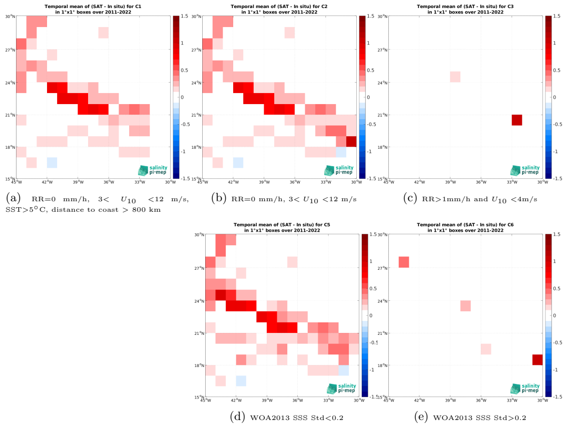
Figure 12: Temporal mean gridded over spatial boxes of size 1^\circ \times 1^\circ of \Delta SSS (SMAP SSS L4 OI v2 - Monthly (IPRC) - TSG (SAMOS)) for 5 different subdatasets corresponding to: RR=0 mm/h, 3 < U_{10} < 12 m/s, SST > 5^\circ\text{C} , distance to coast > 800 km (a), RR=0 mm/h, 3 < U_{10} < 12 m/s (b), RR > 1 mm/h and U_{10} < 4 m/s (c), WOA2013 SSS Std < 0.2 (d), WOA2013 SSS Std > 0.2 (e).
