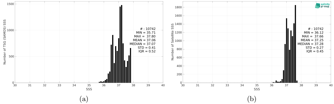
Figure 2: Histograms of SSS from TSG (SAMOS) (a) and SMAP SSS L4 OI v2 - Monthly (IPRC) (b) considering all match-up pairs per bins of 0.1 over the SPURS 1 Pi-MEP region and for the full satellite product period.
