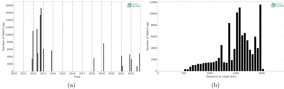
Figure 1: Number of match-ups between TSG (SAMOS) and SMAP SSS L4 OI v2 - Monthly (IPRC) SSS as a function of time (a) and as function of the distance to coast (b) over the SPURS 1 Pi-MEP region and for the full satellite product period.
