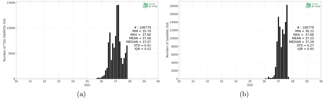
Figure 2: Histograms of SSS from TSG (SAMOS) (a) and SMAP SSS L4 OI v2 - Monthly (IPRC) (b) considering all match-up pairs per bins of 0.1 over the SPURS 1 Pi-MEP region and for the full satellite product period.
