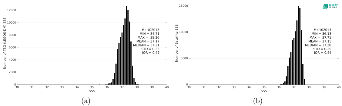
Figure 2: Histograms of SSS from TSG (LEGOS-DM) (a) and SMAP SSS L4 OI v2 - Monthly (IPRC) (b) considering all match-up pairs per bins of 0.1 over the SPURS 1 Pi-MEP region and for the full satellite product period.
