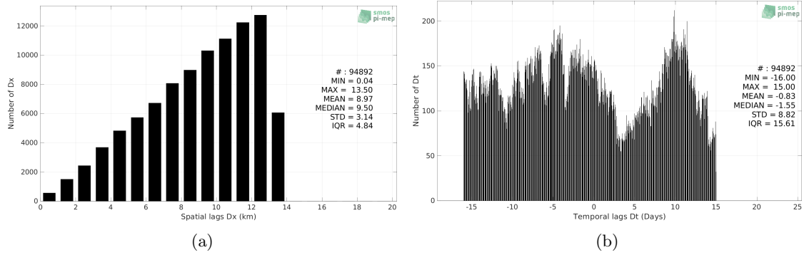
Figure 5: Histograms of the spatial (a) and temporal (b) lags between the location/time of the TSG (LEGOS-DM) measurement and the date of the corresponding SMAP SSS L4 OI v2 - Monthly (IPRC) SSS pixel.
