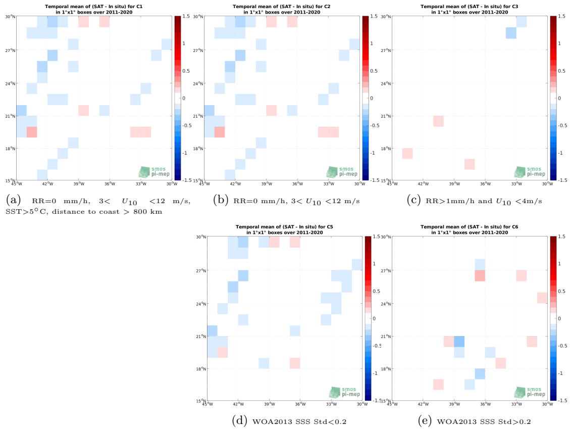
Figure 12: Temporal mean gridded over spatial boxes of size 1^\circ \times 1^\circ of \Delta SSS (SMAP SSS L4 OI v2 - Monthly (IPRC) - TSG (LEGOS-DM)) for 5 different subdatasets corresponding to:RR=0 mm/h, 3 < U_{10} < 12 m/s, SST >5^\circ C, distance to coast > 800 km (a), RR=0 mm/h, 3 < U_{10} < 12 m/s (b), RR >1 mm/h and U_{10} < 4 m/s (c), WOA2013 SSS Std <0.2 (d), WOA2013 SSS Std >0.2 (e).
