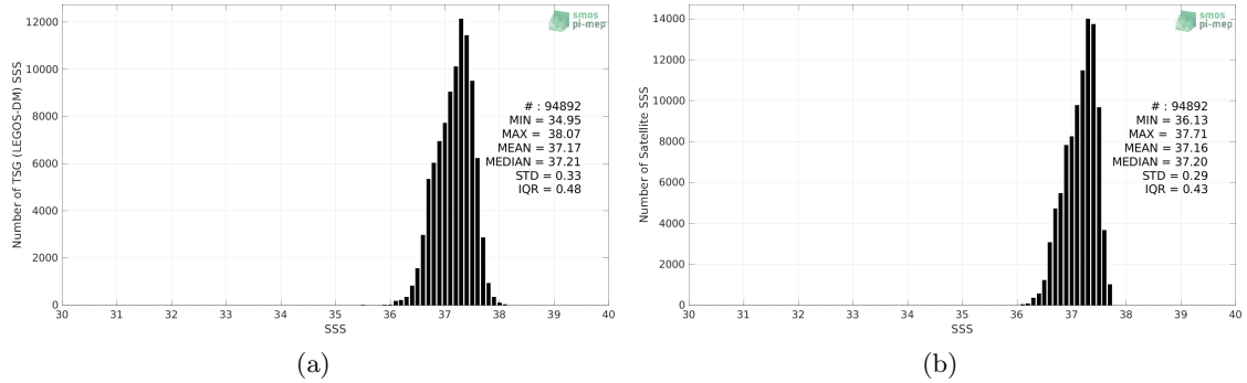
Figure 2: Histograms of SSS from TSG (LEGOS-DM) (a) and SMAP SSS L4 OI v2 - Monthly (IPRC) (b) considering all match-up pairs per bins of 0.1 over the SPURS 1 Pi-MEP region and for the full satellite product period.
