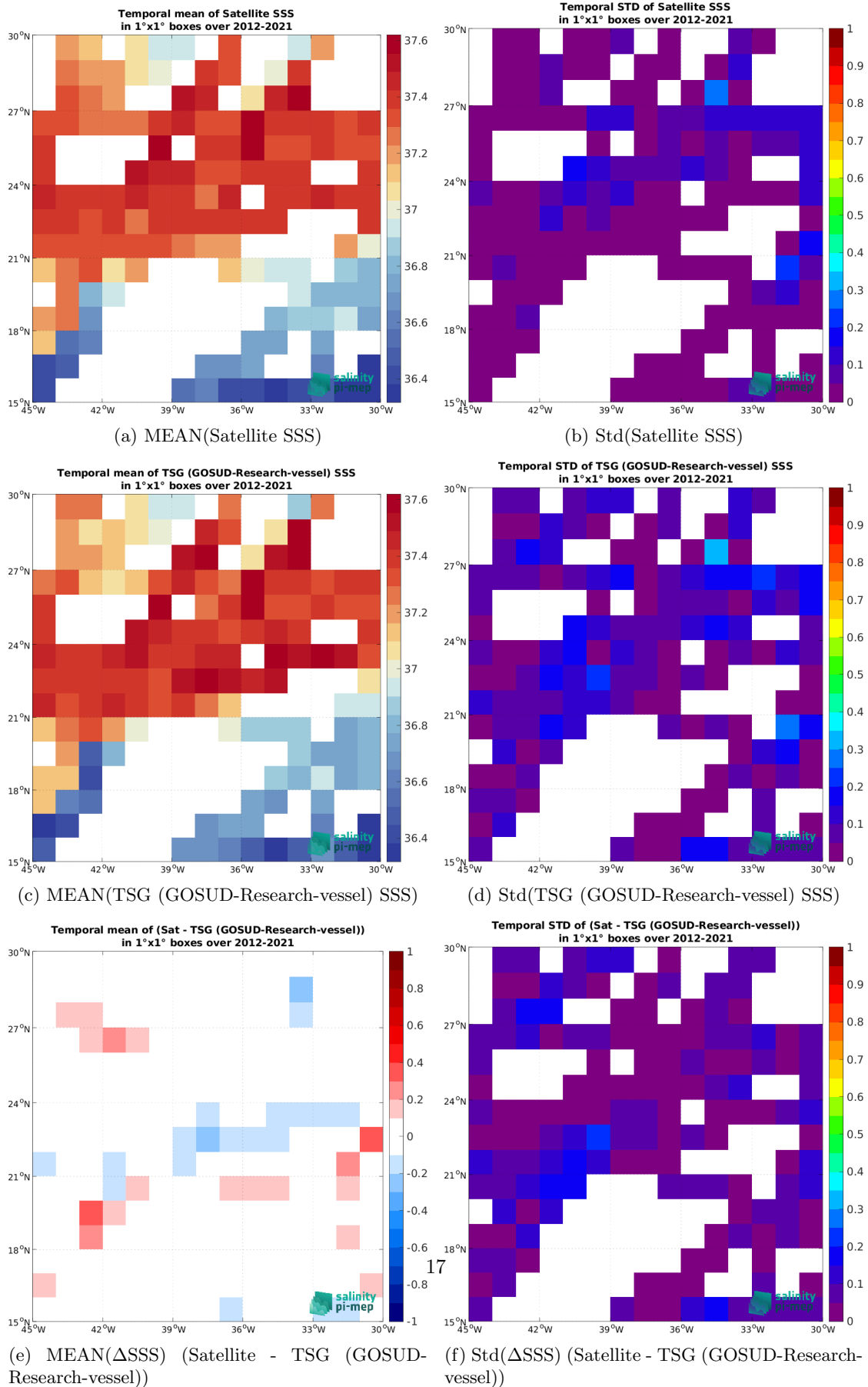
Figure 6: Temporal mean (left) and Std (right) of SSS from SMAP SSS L4 OI v2 - Monthly (IPRC) (top), TSG (GOSUD-Research-vessel) (middle), and of \Delta SSS (Satellite - TSG (GOSUD-Research-vessel)). Only match-up pairs are used to generate these maps.
