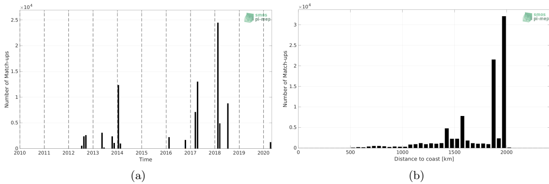
Figure 1: Number of match-ups between TSG (GOSUD-Research-vessel) and SMAP SSS L4 OI v2 - Monthly (IPRC) SSS as a function of time (a) and as function of the distance to coast (b) over the SPURS 1 Pi-MEP region and for the full satellite product period.
