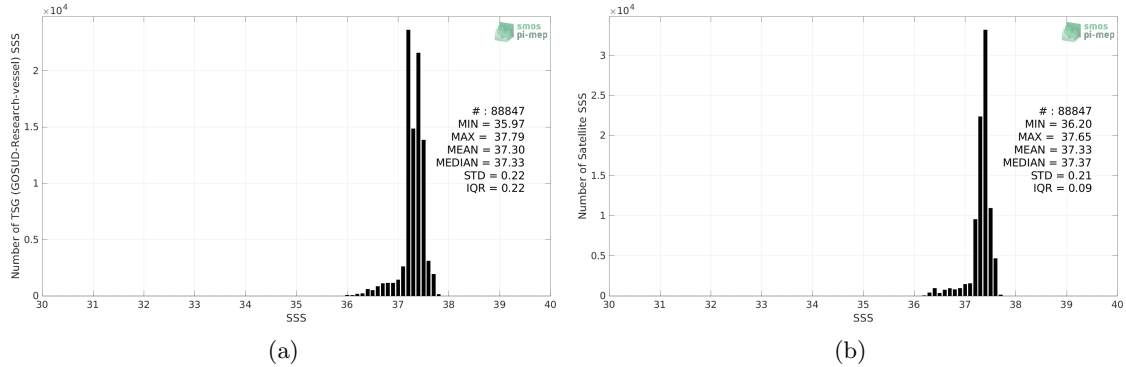
Figure 2: Histograms of SSS from TSG (GOSUD-Research-vessel) (a) and SMAP SSS L4 OI v2 - Monthly (IPRC) (b) considering all match-up pairs per bins of 0.1 over the SPURS 1 Pi-MEP region and for the full satellite product period.
