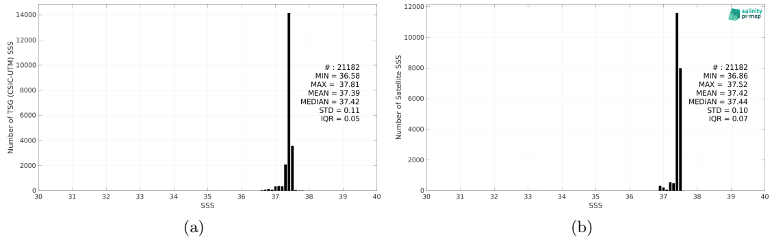
Figure 2: Histograms of SSS from TSG (CSIC-UTM) (a) and SMAP SSS L4 OI v2 - Monthly (IPRC) (b) considering all match-up pairs per bins of 0.1 over the SPURS 1 Pi-MEP region and for the full satellite product period.
