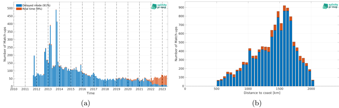
Figure 1: Number of match-ups between Argo and SMAP SSS L4 OI v2 - Monthly (IPRC) SSS as a function of time (a) and as function of the distance to coast (b) over the SPURS 1 Pi-MEP region and for the full satellite product period.
