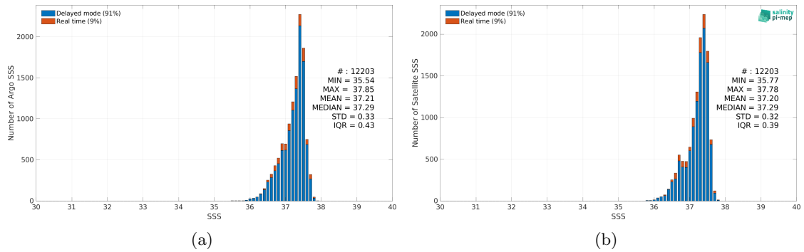
Figure 2: Histograms of SSS from Argo (a) and SMAP SSS L4 OI v2 - Monthly (IPRC) (b) considering all match-up pairs per bins of 0.1 over the SPURS 1 Pi-MEP region and for the full satellite product period.
