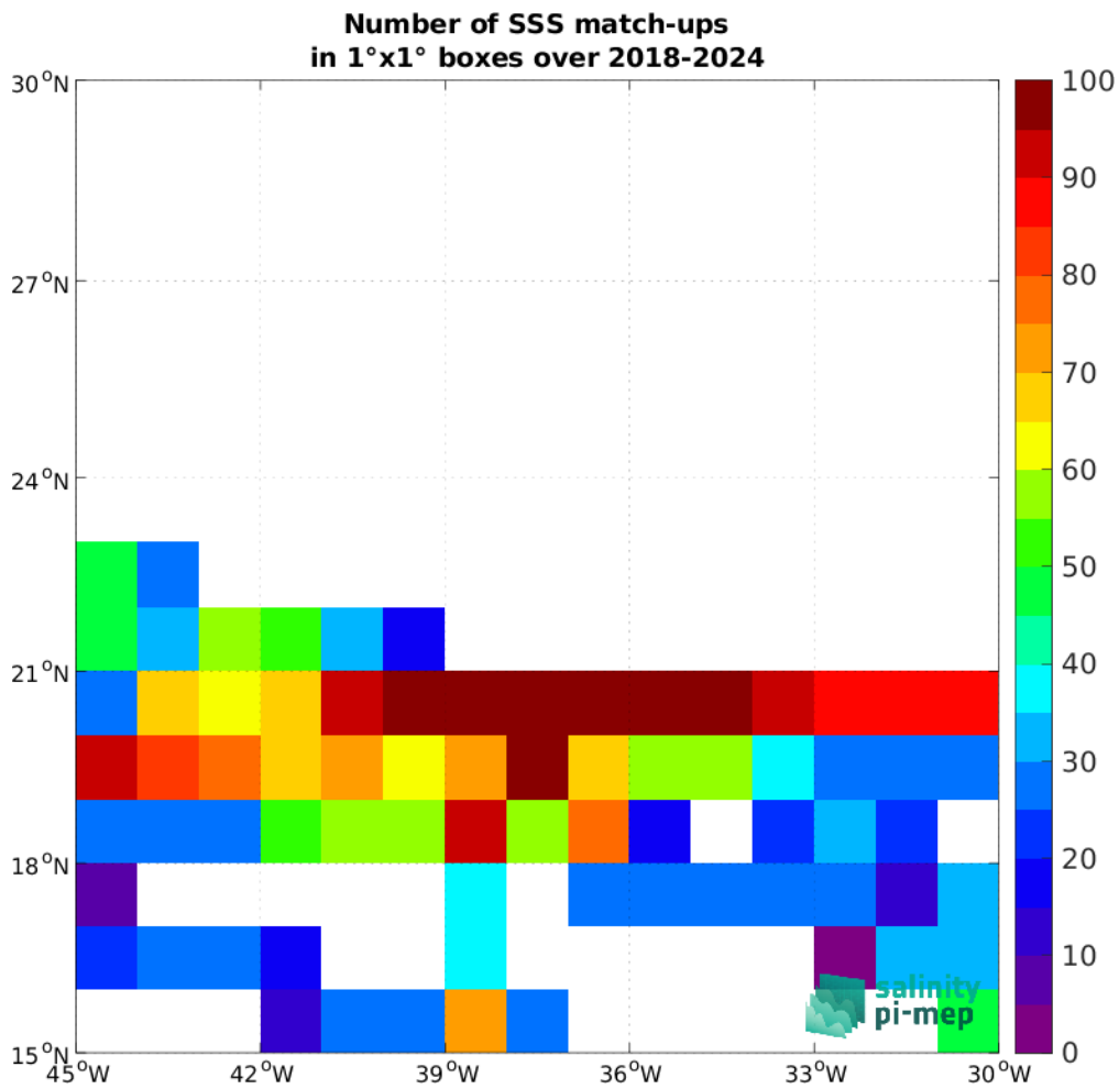
Figure 5: Number of SSS match-ups between TSG (SAMOS) SSS and the SMAP SSS L3 v6 - 8-Day running (RSS) SSS product for the SPURS 1 Pi-MEP region over 1°x1° boxes and for the full satellite product period.
