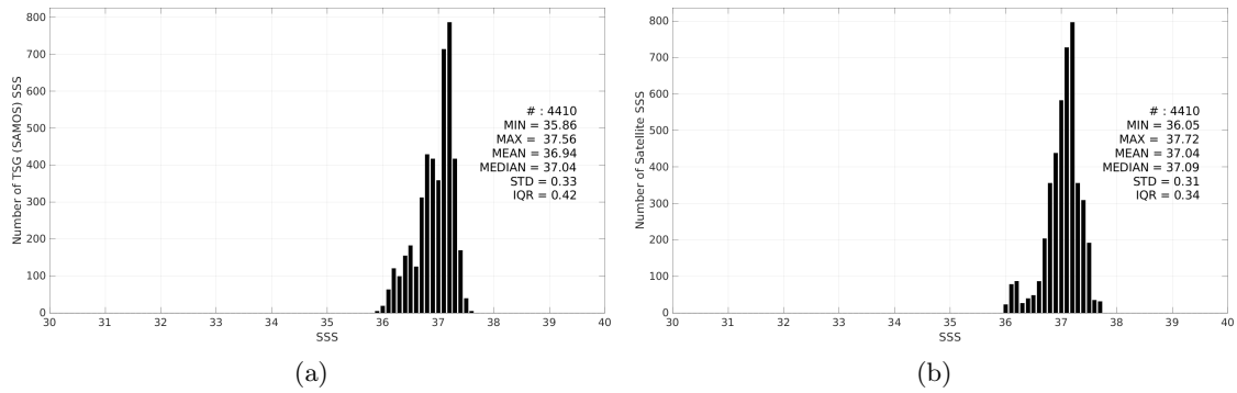
Figure 3: Histograms of SSS from TSG (SAMOS) (a) and SMAP SSS L3 v6 - 8-Day running (RSS) (b) considering all match-up pairs per bins of 0.1 over the SPURS 1 Pi-MEP region and for the full satellite product period.
