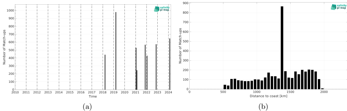
Figure 2: Number of match-ups between TSG (SAMOS) and SMAP SSS L3 v6 - 8-Day running (RSS) SSS as a function of time (a) and as function of the distance to coast (b) over the SPURS 1 Pi-MEP region and for the full satellite product period.
