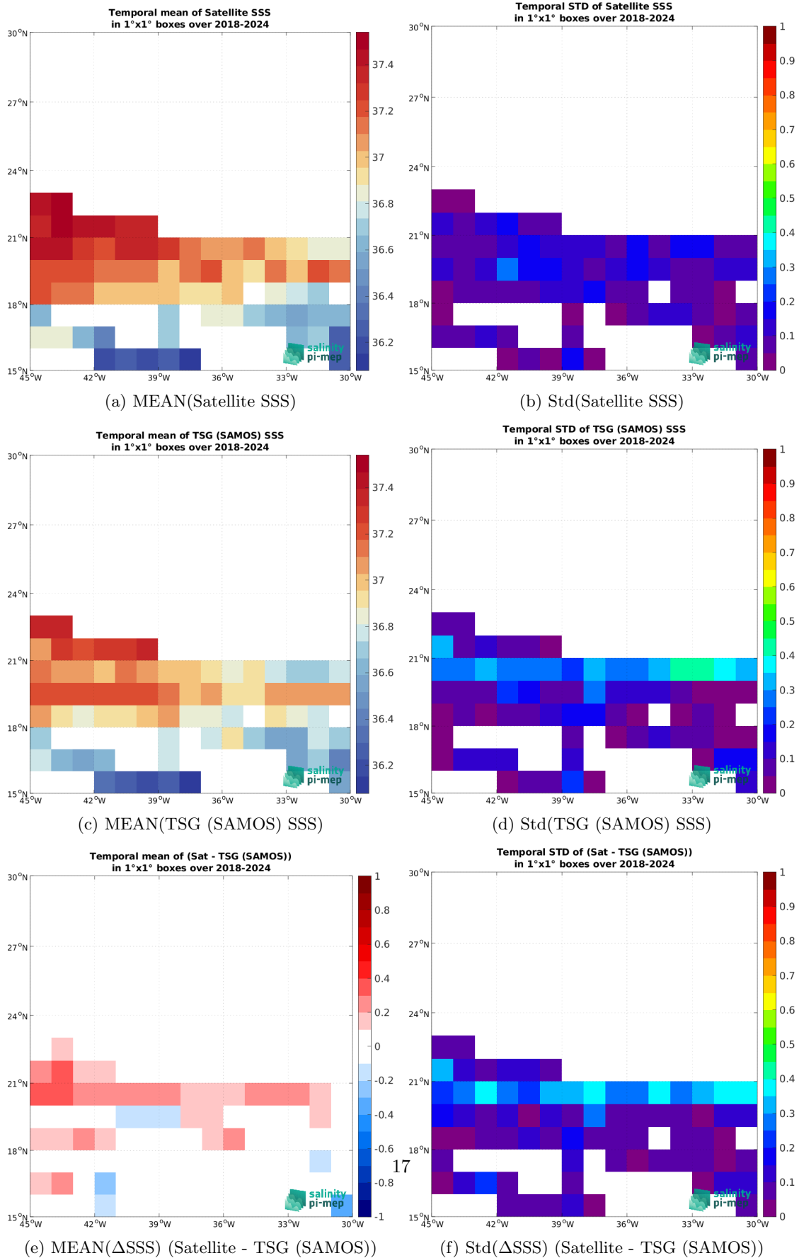
Figure 7: Temporal mean (left) and Std (right) of SSS from SMAP SSS L3 v6 - 8-Day running (RSS) (top), TSG (SAMOS) (middle), and of \Delta SSS (Satellite - TSG (SAMOS)). Only match-up pairs are used to generate these maps.
