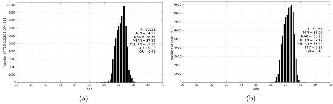
Figure 3: Histograms of SSS from TSG (LEGOS-DM) (a) and SMAP SSS L3 v6 - 8-Day running (RSS) (b) considering all match-up pairs per bins of 0.1 over the SPURS 1 Pi-MEP region and for the full satellite product period.
