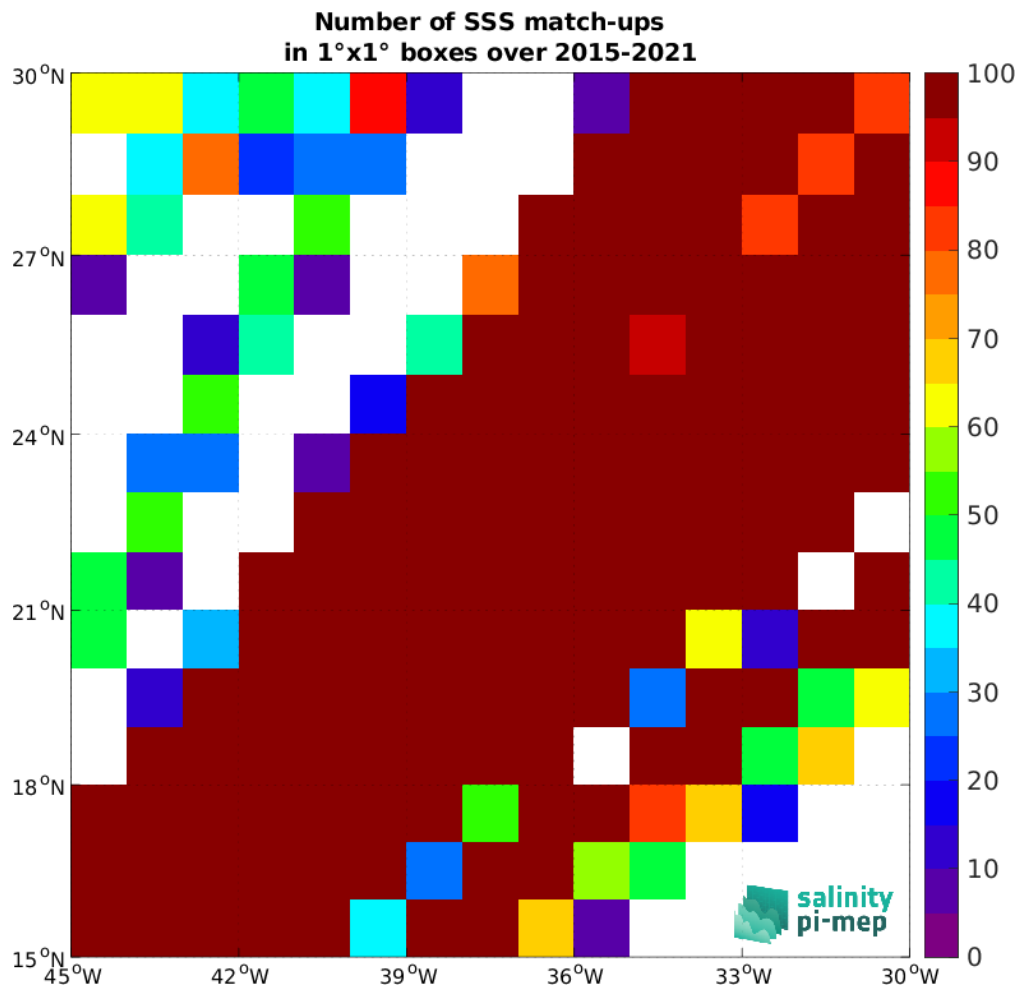
Figure 5: Number of SSS match-ups between TSG (LEGOS-DM) SSS and the SMAP SSS L3 v6 - 8-Day running (RSS) SSS product for the SPURS 1 Pi-MEP region over 1^\circ \times 1^\circ boxes and for the full satellite product period.
