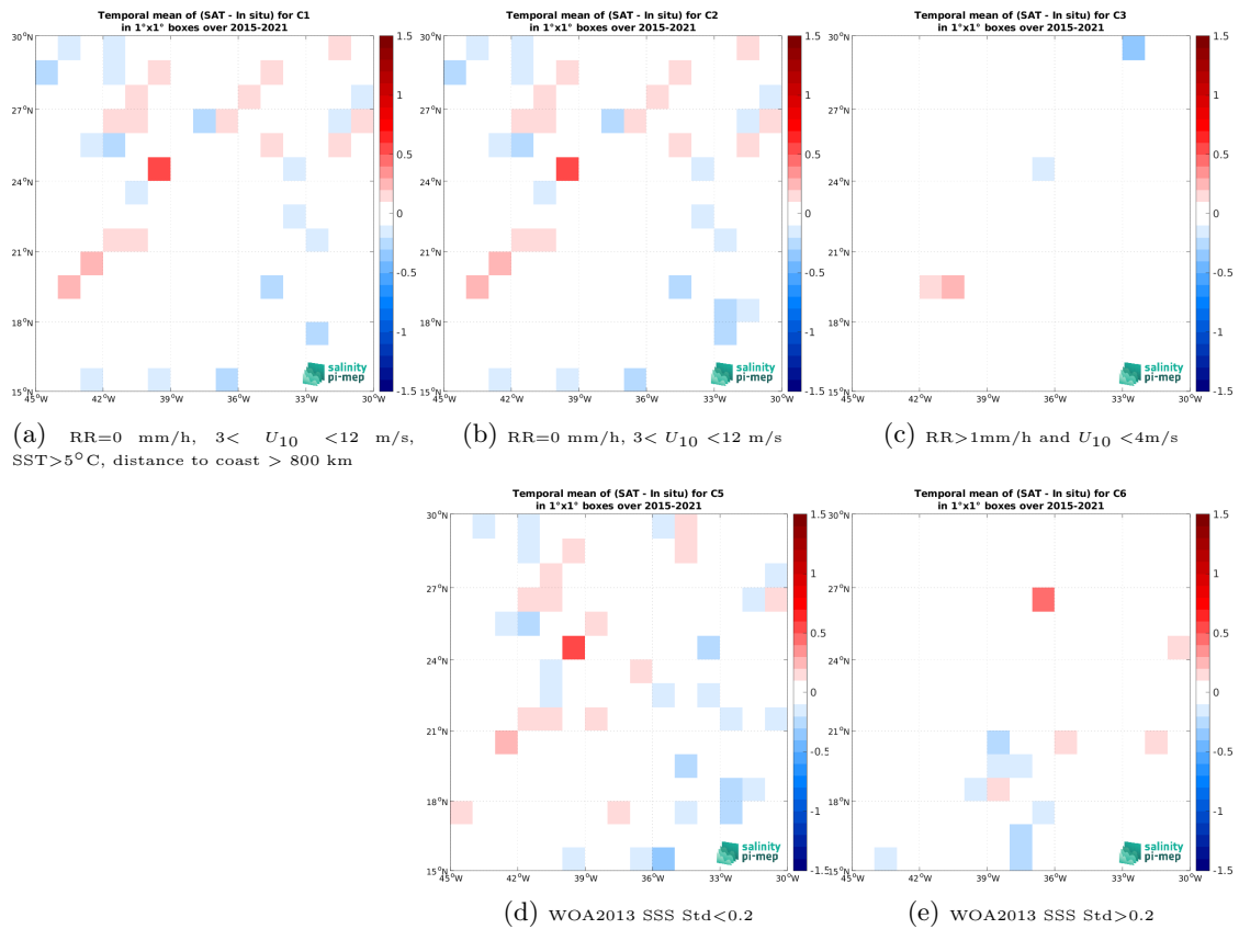
Figure 14: Temporal mean gridded over spatial boxes of size 1^\circ \times 1^\circ of \Delta SSS (SMAP SSS L3 v6 - 8-Day running (RSS) - TSG (LEGOS-DM)) for 5 different subdatasets corresponding to: RR=0 mm/h, 3 < U_{10} < 12 m/s, SST > 5^\circ C , distance to coast > 800 km (a), RR=0 mm/h, 3 < U_{10} < 12 m/s (b), RR > 1 mm/h and U_{10} < 4 m/s (c), WOA2013 SSS Std < 0.2 (d), WOA2013 SSS Std > 0.2 (e).
