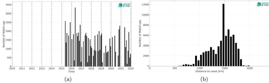
Figure 2: Number of match-ups between TSG (LEGOS-DM) and SMAP SSS L3 v6 - 8-Day running (RSS) SSS as a function of time (a) and as function of the distance to coast (b) over the SPURS 1 Pi-MEP region and for the full satellite product period.
