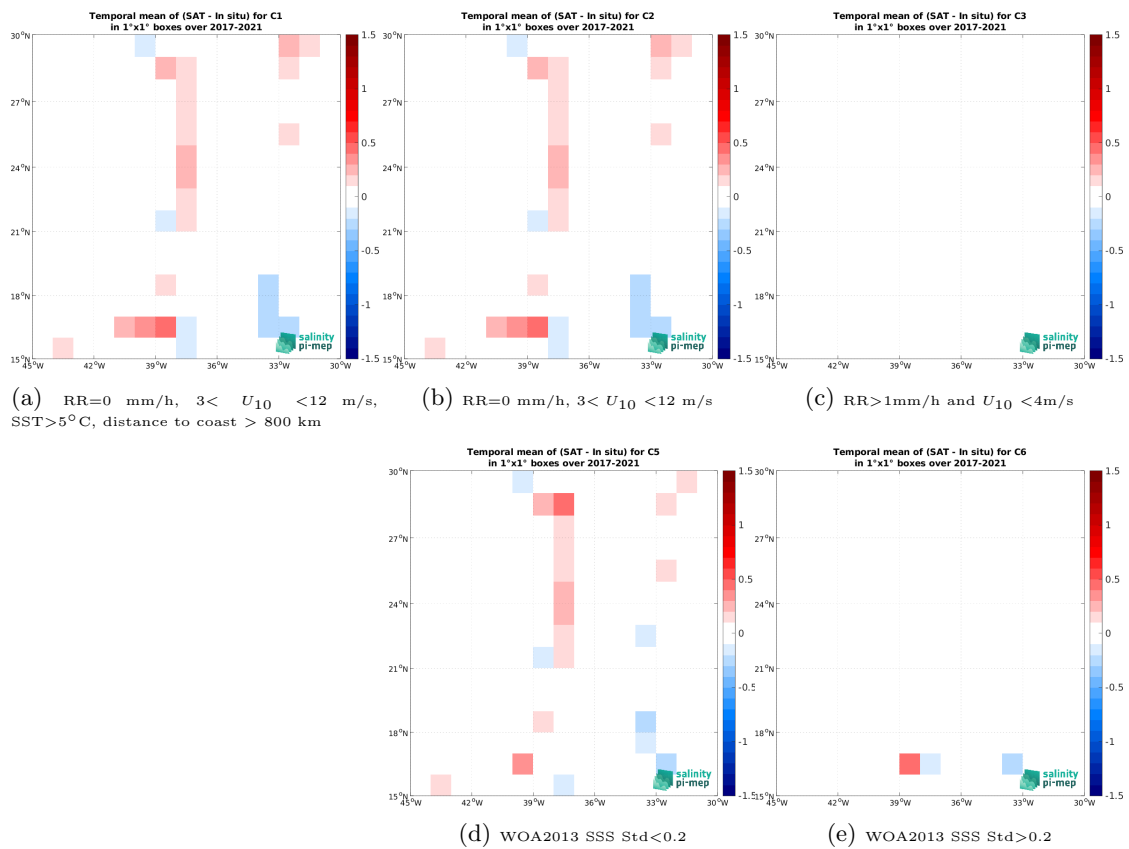
Figure 14: Temporal mean gridded over spatial boxes of size 1^\circ \times 1^\circ of \Delta SSS (SMAP SSS L3 v6 - 8-Day running (RSS) - TSG (GOSUD-Sailing-ship)) for 5 different subdatasets corresponding to:RR=0 mm/h, 3 < U_{10} < 12 m/s, SST >5^\circ C, distance to coast > 800 km (a), RR=0 mm/h, 3 < U_{10} < 12 m/s (b), RR >1 mm/h and U_{10} < 4 m/s (c), WOA2013 SSS Std <0.2 (d), WOA2013 SSS Std >0.2 (e).
