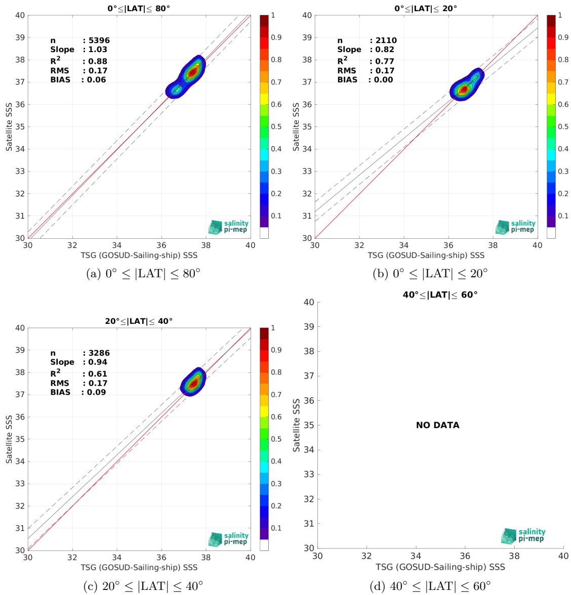
Figure 10: Contour maps of the concentration of SMAP SSS L3 v6 - 8-Day running (RSS) SSS (y-axis) versus TSG (GOSUD-Sailing-ship) SSS (x-axis) at match-up pairs for different latitude bands. For each plot, the red line shows x=y . The black thin and dashed lines indicate a linear fit through the data cloud and the \pm 95\% confidence levels, respectively. The number match-up pairs n , the slope and R^2 coefficient of the linear fit, the root mean square (RMS) and the mean bias between satellite and in situ data are indicated for each latitude band in each plots.
