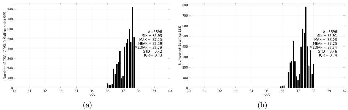
Figure 3: Histograms of SSS from TSG (GOSUD-Sailing-ship) (a) and SMAP SSS L3 v6 - 8-Day running (RSS) (b) considering all match-up pairs per bins of 0.1 over the SPURS 1 Pi-MEP region and for the full satellite product period.
