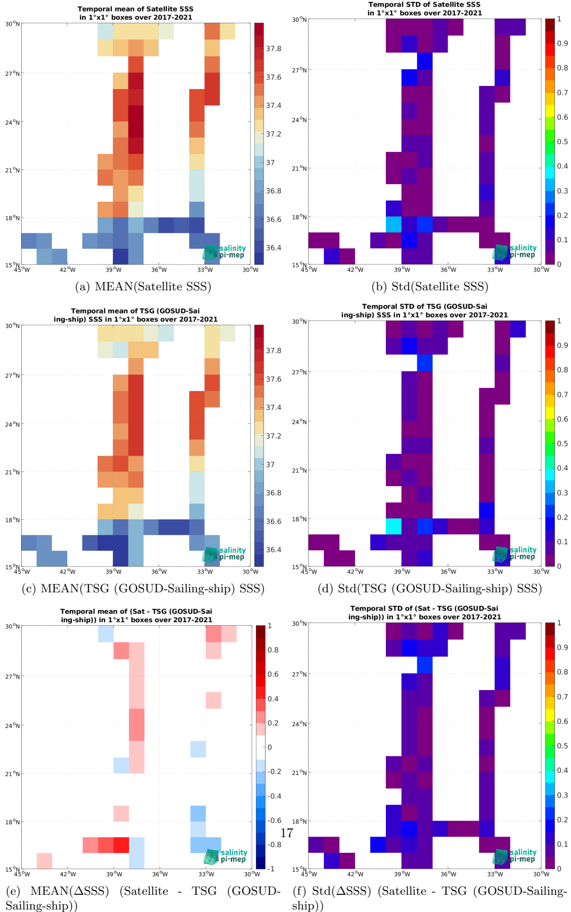
Figure 7: Temporal mean (left) and Std (right) of SSS from SMAP SSS L3 v6 - 8-Day running (RSS) (top), TSG (GOSUD-Sailing-ship) (middle), and of \Delta SSS (Satellite - TSG (GOSUD-Sailing-ship)). Only match-up pairs are used to generate these maps.
