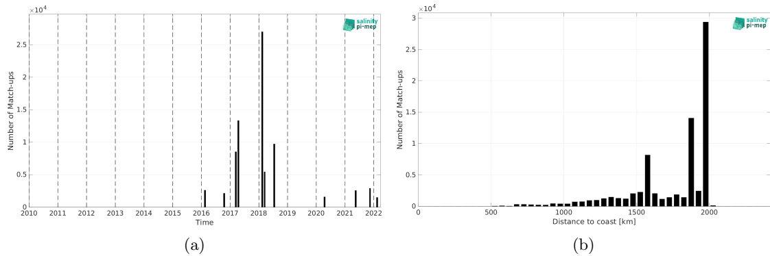
Figure 2: Number of match-ups between TSG (GOSUD-Research-vessel) and SMAP SSS L3 v6 - 8-Day running (RSS) SSS as a function of time (a) and as function of the distance to coast (b) over the SPURS 1 Pi-MEP region and for the full satellite product period.
