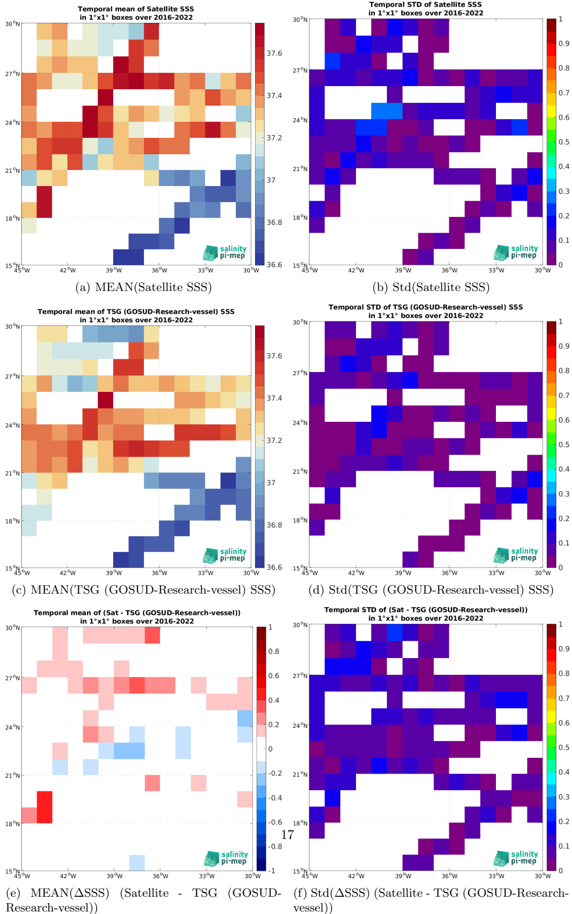
Figure 7: Temporal mean (left) and Std (right) of SSS from SMAP SSS L3 v6 - 8-Day running (RSS) (top), TSG (GOSUD-Research-vessel) (middle), and of \Delta SSS (Satellite - TSG (GOSUD-Research-vessel)). Only match-up pairs are used to generate these maps.
