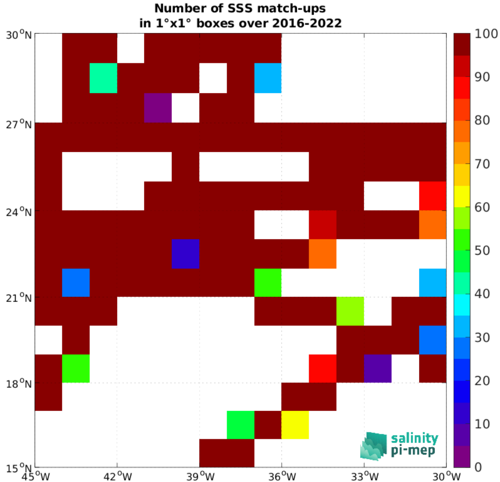
Figure 5: Number of SSS match-ups between TSG (GOSUD-Research-vessel) SSS and the SMAP SSS L3 v6 - 8-Day running (RSS) SSS product for the SPURS 1 Pi-MEP region over 1^\circ \times 1^\circ boxes and for the full satellite product period.
