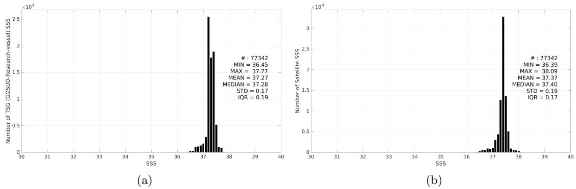
Figure 3: Histograms of SSS from TSG (GOSUD-Research-vessel) (a) and SMAP SSS L3 v6 - 8-Day running (RSS) (b) considering all match-up pairs per bins of 0.1 over the SPURS 1 Pi-MEP region and for the full satellite product period.
