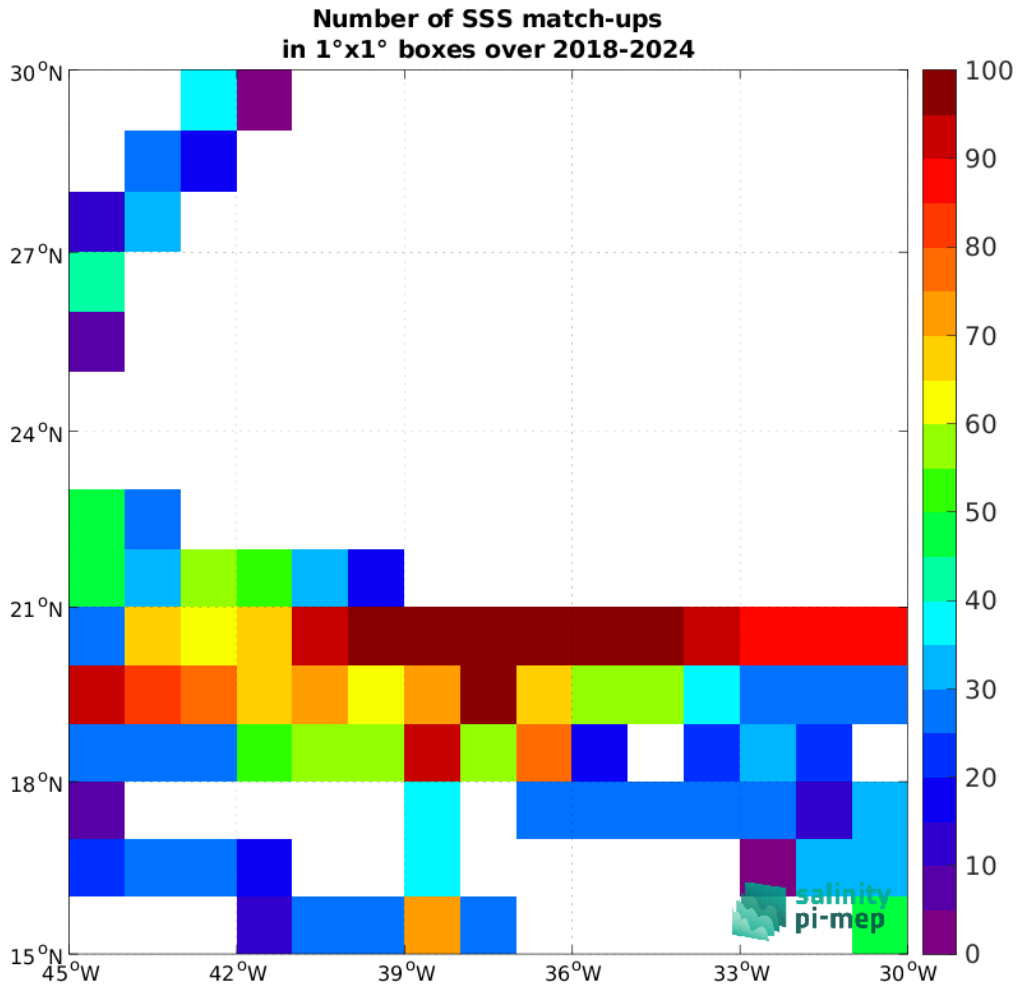
Figure 5: Number of SSS match-ups between TSG (SAMOS) SSS and the SMAP SSS L3 v6 - Monthly (RSS) SSS product for the SPURS 1 Pi-MEP region over 1^\circ \times 1^\circ boxes and for the full satellite product period.
