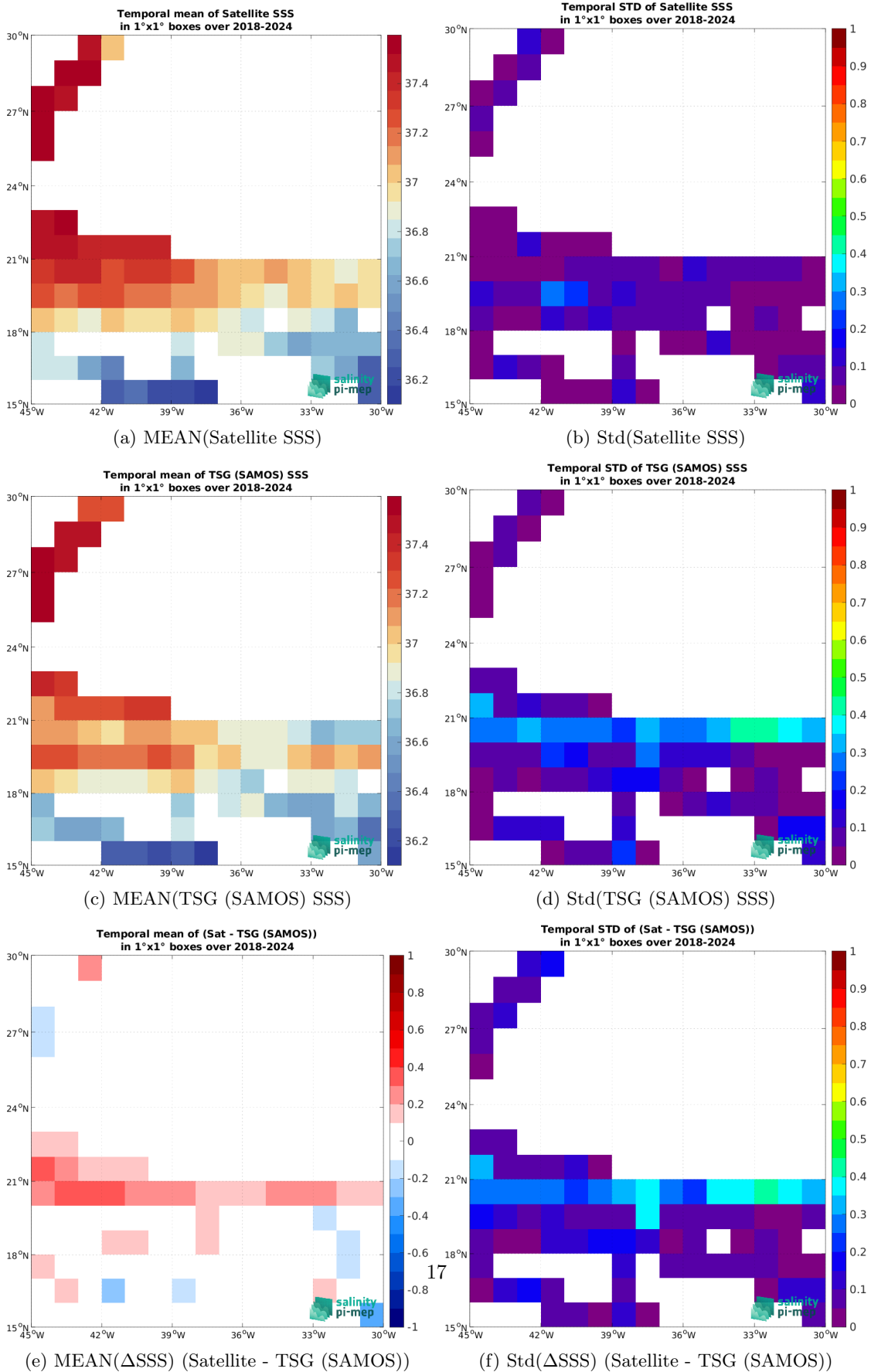
Figure 7: Temporal mean (left) and Std (right) of SSS from SMAP SSS L3 v6 - Monthly (RSS) (top), TSG (SAMOS) (middle), and of \Delta SSS (Satellite - TSG (SAMOS)). Only match-up pairs are used to generate these maps.
