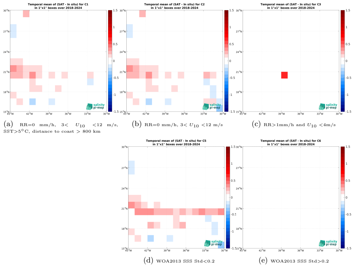
Figure 14: Temporal mean gridded over spatial boxes of size 1^\circ \times 1^\circ of \Delta SSS (SMAP SSS L3 v6 - Monthly (RSS) - TSG (SAMOS)) for 5 different subdatasets corresponding to: RR=0 mm/h, 3 < U_{10} < 12 m/s, SST > 5^\circ C , distance to coast > 800 km (a), RR=0 mm/h, 3 < U_{10} < 12 m/s (b), RR > 1 mm/h and U_{10} < 4 m/s (c), WOA2013 SSS Std < 0.2 (d), WOA2013 SSS Std > 0.2 (e).
