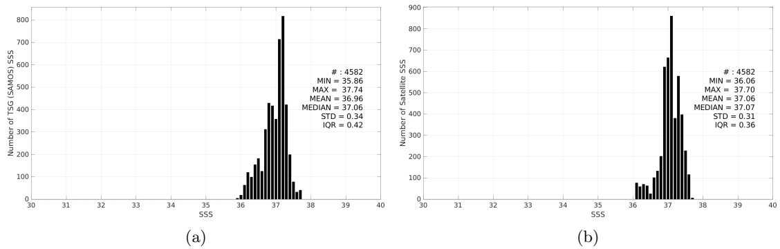
Figure 3: Histograms of SSS from TSG (SAMOS) (a) and SMAP SSS L3 v6 - Monthly (RSS) (b) considering all match-up pairs per bins of 0.1 over the SPURS 1 Pi-MEP region and for the full satellite product period.
