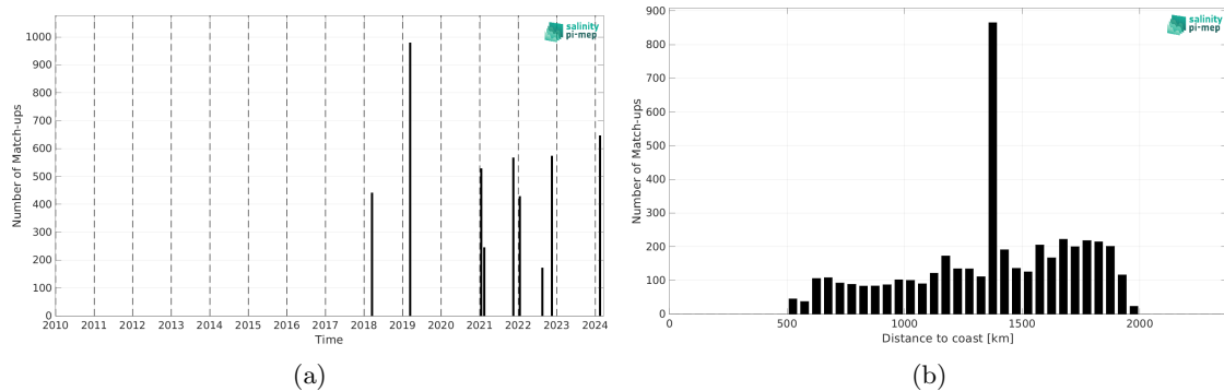
Figure 2: Number of match-ups between TSG (SAMOS) and SMAP SSS L3 v6 - Monthly (RSS) SSS as a function of time (a) and as function of the distance to coast (b) over the SPURS 1 Pi-MEP region and for the full satellite product period.
