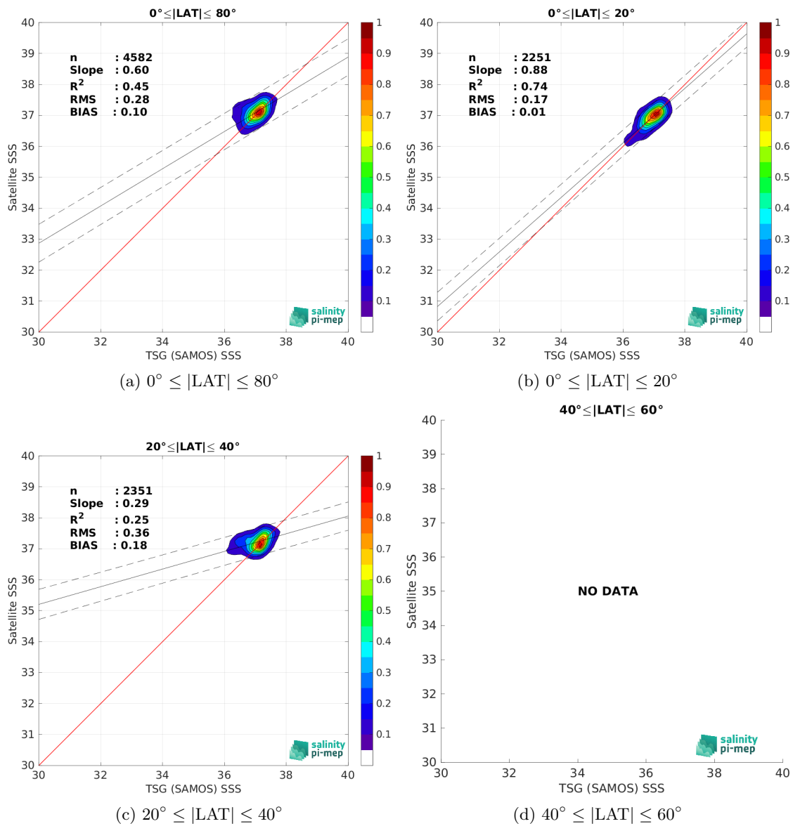
Figure 10: Contour maps of the concentration of SMAP SSS L3 v6 - Monthly (RSS) SSS (y-axis) versus TSG (SAMOS) SSS (x-axis) at match-up pairs for different latitude bands. For each plot, the red line shows x=y . The black thin and dashed lines indicate a linear fit through the data cloud and the \pm 95\% confidence levels, respectively. The number match-up pairs n , the slope and R^2 coefficient of the linear fit, the root mean square (RMS) and the mean bias between satellite and in situ data are indicated for each latitude band in each plots.
