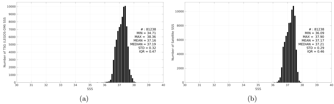
Figure 3: Histograms of SSS from TSG (LEGOS-DM) (a) and SMAP SSS L3 v6 - Monthly (RSS) (b) considering all match-up pairs per bins of 0.1 over the SPURS 1 Pi-MEP region and for the full satellite product period.
