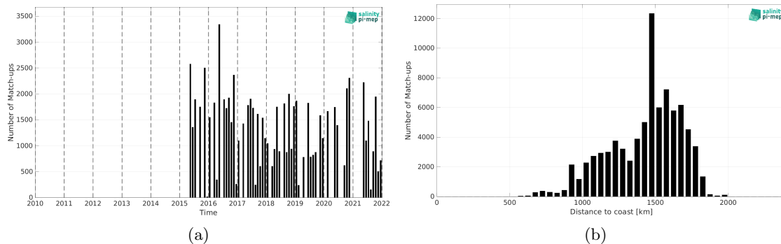
Figure 2: Number of match-ups between TSG (LEGOS-DM) and SMAP SSS L3 v6 - Monthly (RSS) SSS as a function of time (a) and as function of the distance to coast (b) over the SPURS 1 Pi-MEP region and for the full satellite product period.
