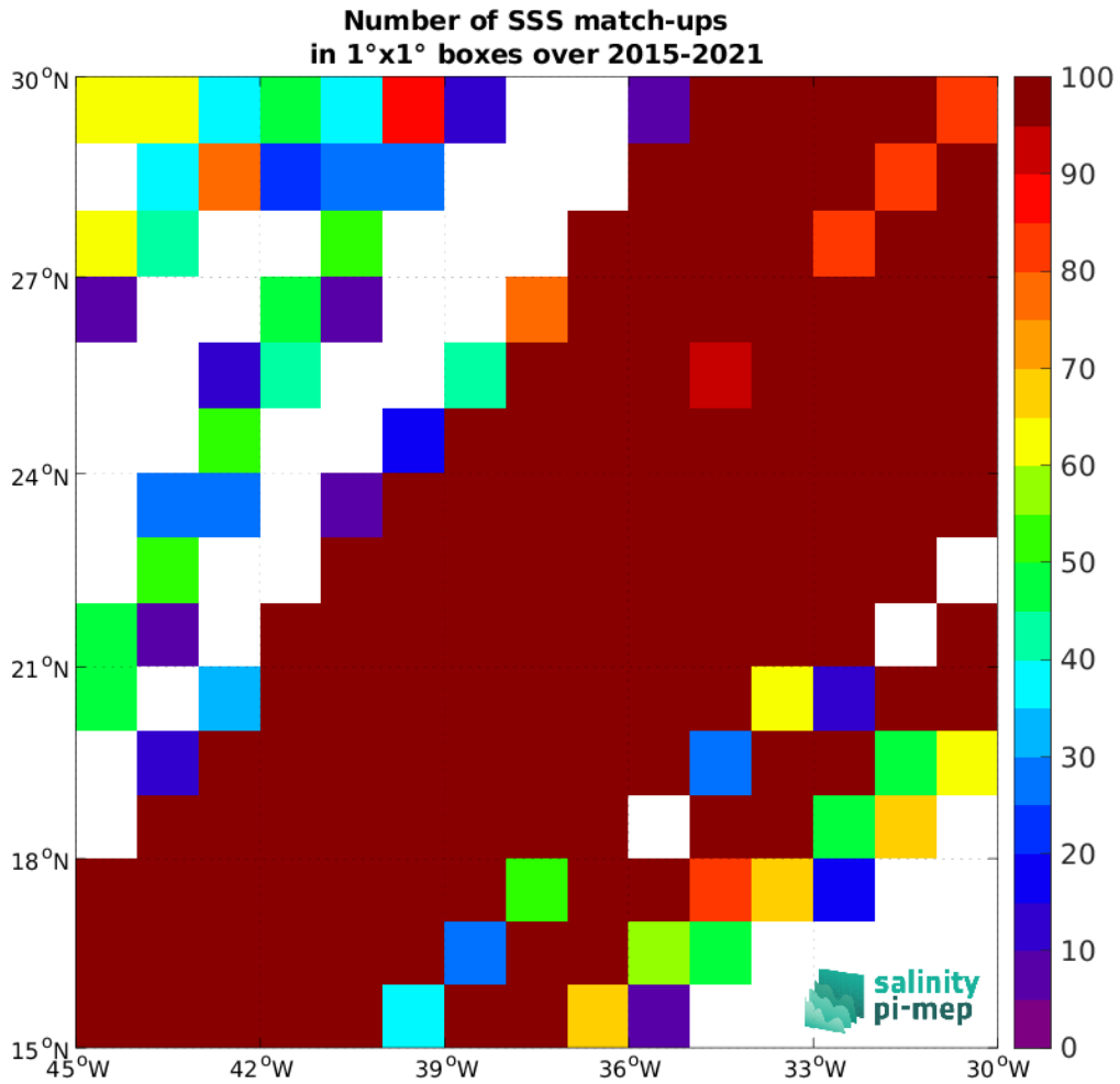
Figure 5: Number of SSS match-ups between TSG (LEGOS-DM) SSS and the SMAP SSS L3 v6 - Monthly (RSS) SSS product for the SPURS 1 Pi-MEP region over 1^\circ \times 1^\circ boxes and for the full satellite product period.
