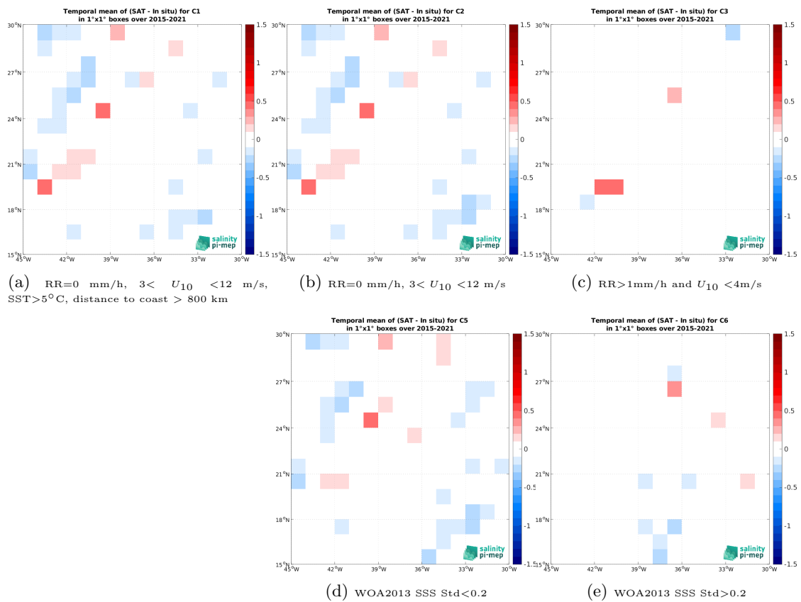
Figure 14: Temporal mean gridded over spatial boxes of size 1^\circ \times 1^\circ of \Delta SSS (SMAP SSS L3 v6 - Monthly (RSS) - TSG (LEGOS-DM)) for 5 different subdatasets corresponding to: RR=0 mm/h, 3 < U_{10} < 12 m/s, SST > 5^\circ C , distance to coast > 800 km (a), RR=0 mm/h, 3 < U_{10} < 12 m/s (b), RR > 1 mm/h and U_{10} < 4 m/s (c), WOA2013 SSS Std < 0.2 (d), WOA2013 SSS Std > 0.2 (e).
