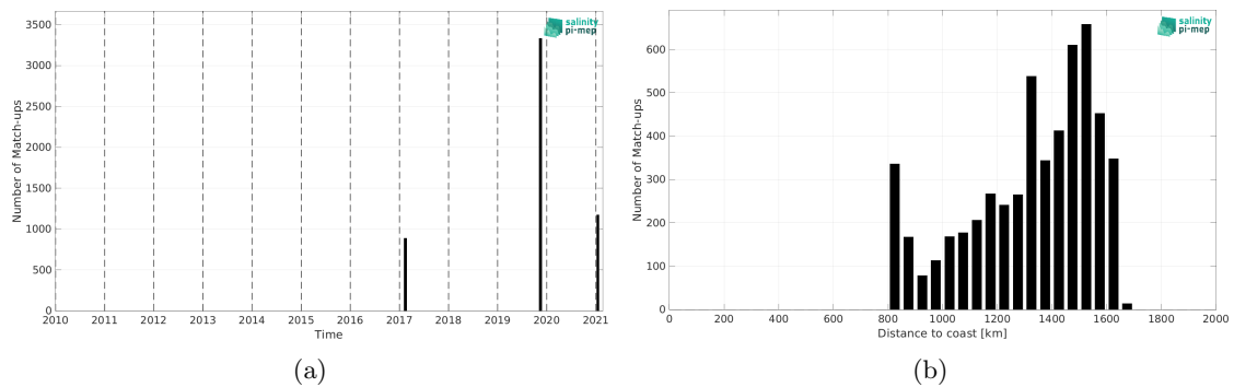
Figure 2: Number of match-ups between TSG (GOSUD-Sailing-ship) and SMAP SSS L3 v6 - Monthly (RSS) SSS as a function of time (a) and as function of the distance to coast (b) over the SPURS 1 Pi-MEP region and for the full satellite product period.
