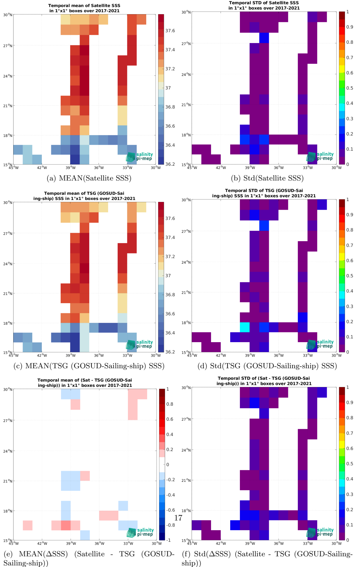
Figure 7: Temporal mean (left) and Std (right) of SSS from SMAP SSS L3 v6 - Monthly (RSS) (top), TSG (GOSUD-Sailing-ship) (middle), and of \Delta SSS (Satellite - TSG (GOSUD-Sailing-ship)). Only match-up pairs are used to generate these maps.
