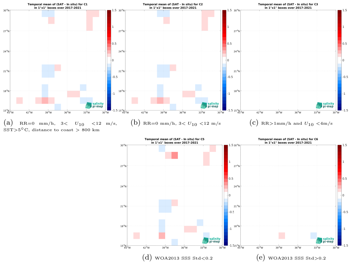
Figure 14: Temporal mean gridded over spatial boxes of size 1^\circ \times 1^\circ of \Delta SSS (SMAP SSS L3 v6 - Monthly (RSS) - TSG (GOSUD-Sailing-ship)) for 5 different subdatasets corresponding to: RR=0 mm/h, 3 < U_{10} < 12 m/s, SST > 5^\circ C , distance to coast > 800 km (a), RR=0 mm/h, 3 < U_{10} < 12 m/s (b), RR > 1 mm/h and U_{10} < 4 m/s (c), WOA2013 SSS Std < 0.2 (d), WOA2013 SSS Std > 0.2 (e).
