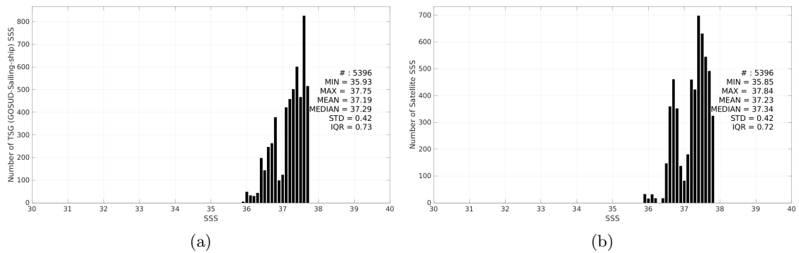
Figure 3: Histograms of SSS from TSG (GOSUD-Sailing-ship) (a) and SMAP SSS L3 v6 - Monthly (RSS) (b) considering all match-up pairs per bins of 0.1 over the SPURS 1 Pi-MEP region and for the full satellite product period.
