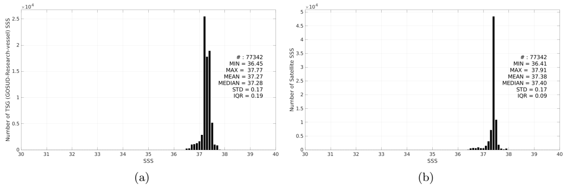
Figure 3: Histograms of SSS from TSG (GOSUD-Research-vessel) (a) and SMAP SSS L3 v6 - Monthly (RSS) (b) considering all match-up pairs per bins of 0.1 over the SPURS 1 Pi-MEP region and for the full satellite product period.
