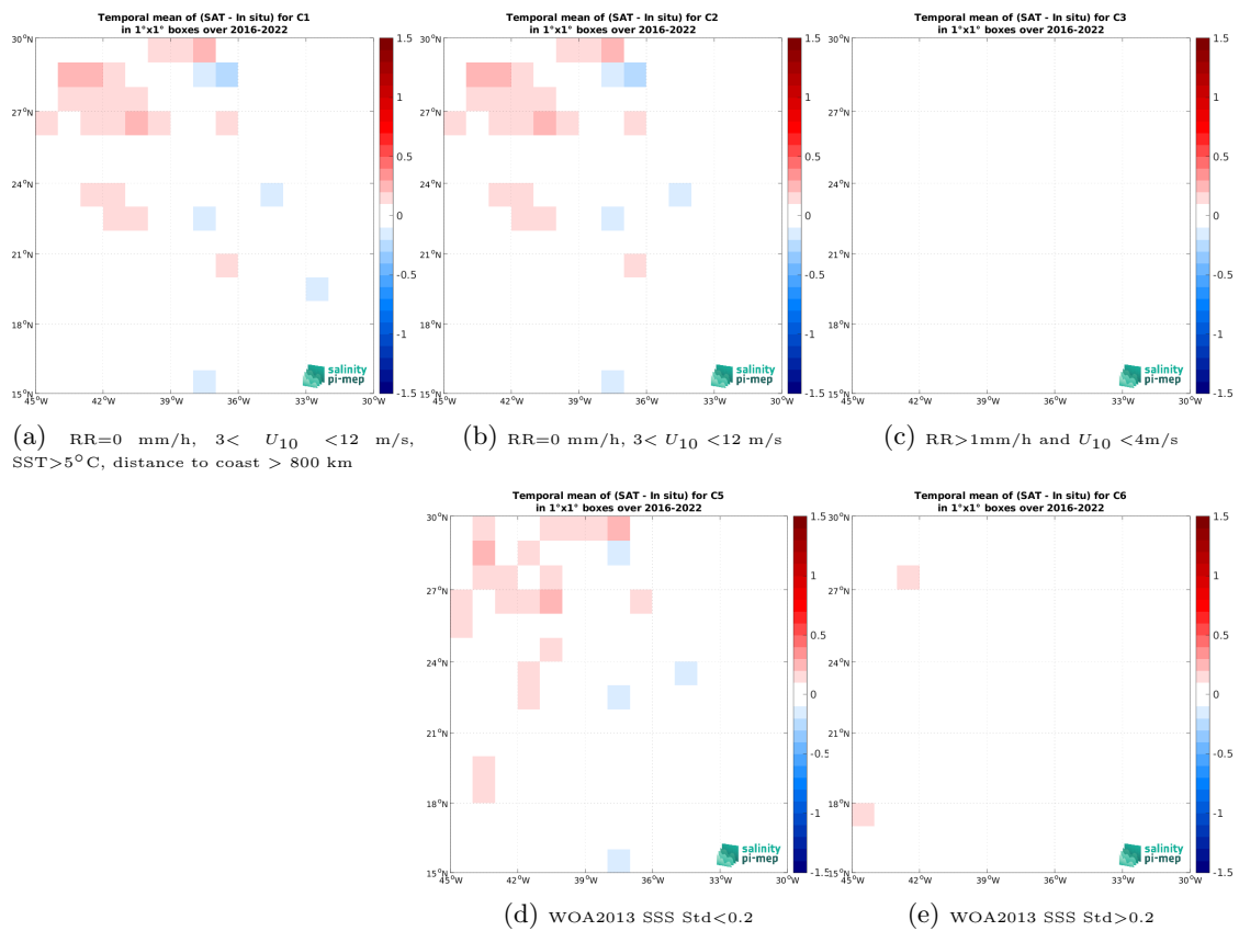
Figure 14: Temporal mean gridded over spatial boxes of size 1^\circ \times 1^\circ of \Delta SSS (SMAP SSS L3 v6 - Monthly (RSS) - TSG (GOSUD-Research-vessel)) for 5 different subdatasets corresponding to:RR=0 mm/h, 3 < U_{10} < 12 m/s, SST>5°C, distance to coast > 800 km (a), RR=0 mm/h, 3 < U_{10} < 12 m/s (b), RR>1mm/h and U_{10} < 4 m/s (c), WOA2013 SSS Std<0.2 (d), WOA2013 SSS Std>0.2 (e).
