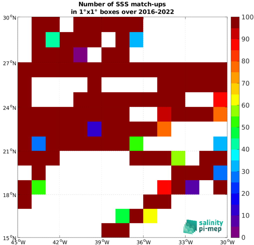
Figure 5: Number of SSS match-ups between TSG (GOSUD-Research-vessel) SSS and the SMAP SSS L3 v6 - Monthly (RSS) SSS product for the SPURS 1 Pi-MEP region over 1^\circ \times 1^\circ boxes and for the full satellite product period.
