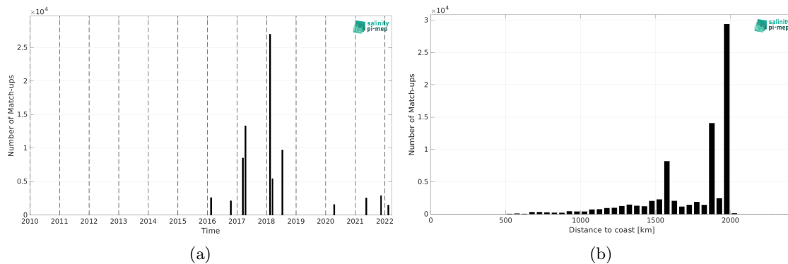
Figure 2: Number of match-ups between TSG (GOSUD-Research-vessel) and SMAP SSS L3 v6 - Monthly (RSS) SSS as a function of time (a) and as function of the distance to coast (b) over the SPURS 1 Pi-MEP region and for the full satellite product period.
