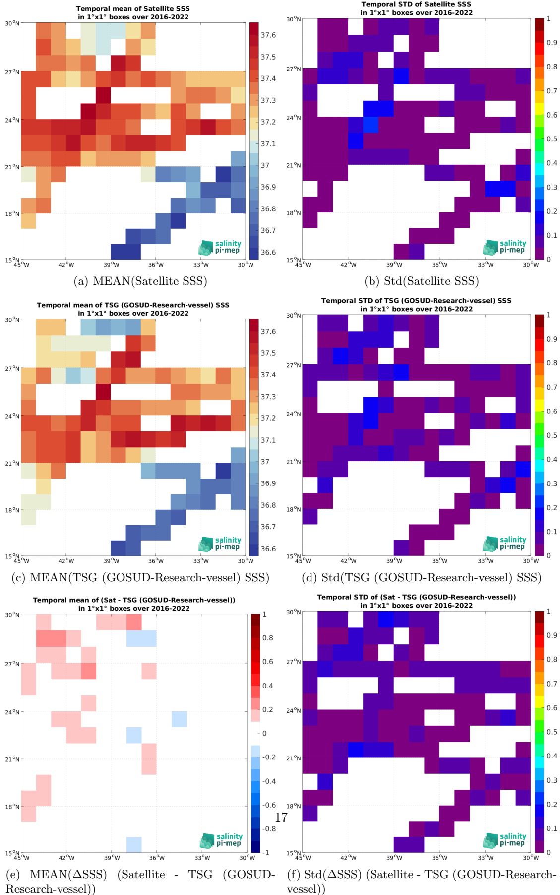
Figure 7: Temporal mean (left) and Std (right) of SSS from SMAP SSS L3 v6 - Monthly (RSS) (top), TSG (GOSUD-Research-vessel) (middle), and of \Delta SSS (Satellite - TSG (GOSUD-Research-vessel)). Only match-up pairs are used to generate these maps.
