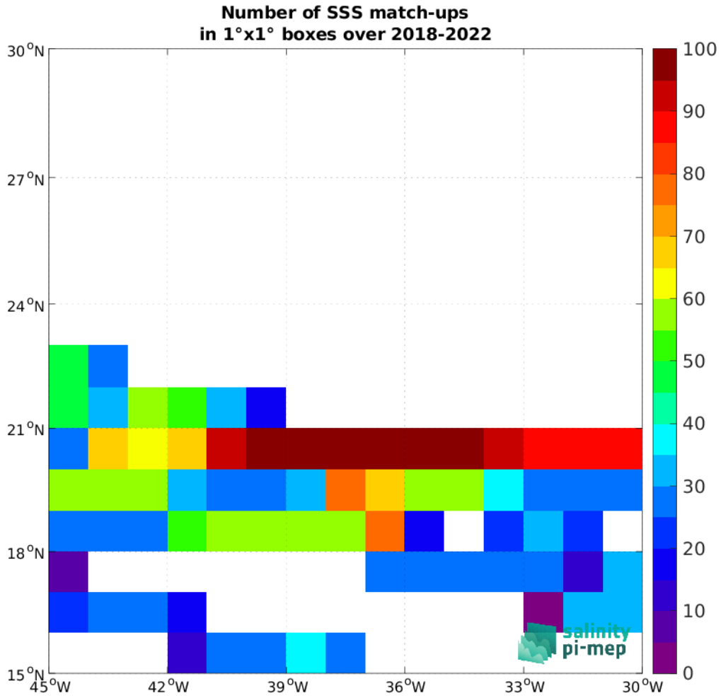
Figure 5: Number of SSS match-ups between TSG (SAMOS) SSS and the SMAP SSS L3 v5.3 - 8-Day running (RSS) SSS product for the SPURS 1 Pi-MEP region over 1°x1° boxes and for the full satellite product period.
