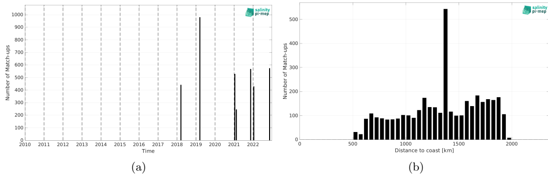
Figure 2: Number of match-ups between TSG (SAMOS) and SMAP SSS L3 v5.3 - 8-Day running (RSS) SSS as a function of time (a) and as function of the distance to coast (b) over the SPURS 1 Pi-MEP region and for the full satellite product period.
