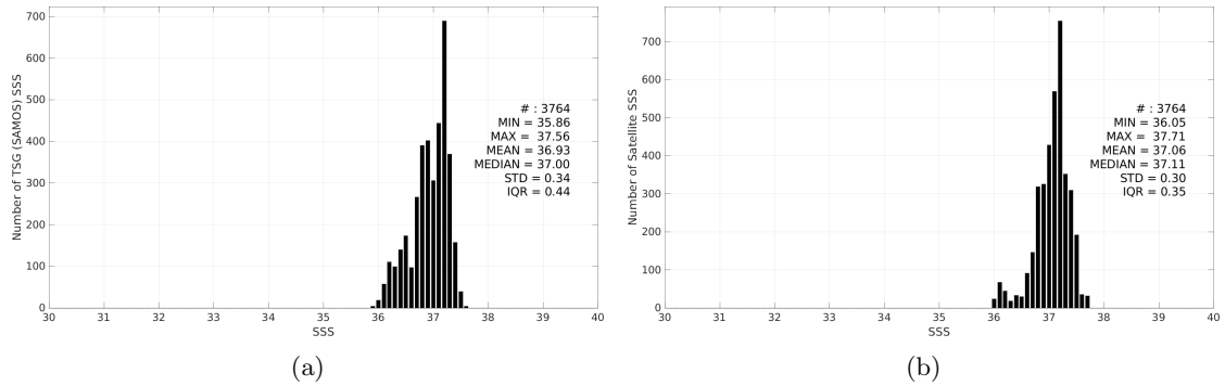
Figure 3: Histograms of SSS from TSG (SAMOS) (a) and SMAP SSS L3 v5.3 - 8-Day running (RSS) (b) considering all match-up pairs per bins of 0.1 over the SPURS 1 Pi-MEP region and for the full satellite product period.
