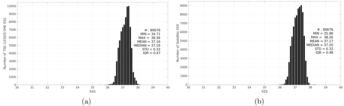
Figure 3: Histograms of SSS from TSG (LEGOS-DM) (a) and SMAP SSS L3 v5.3 - 8-Day running (RSS) (b) considering all match-up pairs per bins of 0.1 over the SPURS 1 Pi-MEP region and for the full satellite product period.
