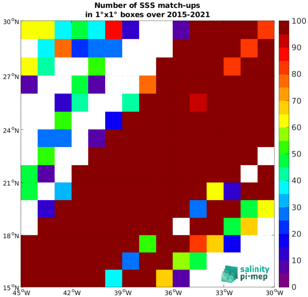
Figure 5: Number of SSS match-ups between TSG (LEGOS-DM) SSS and the SMAP SSS L3 v5.3 - 8-Day running (RSS) SSS product for the SPURS 1 Pi-MEP region over 1°x1° boxes and for the full satellite product period.
