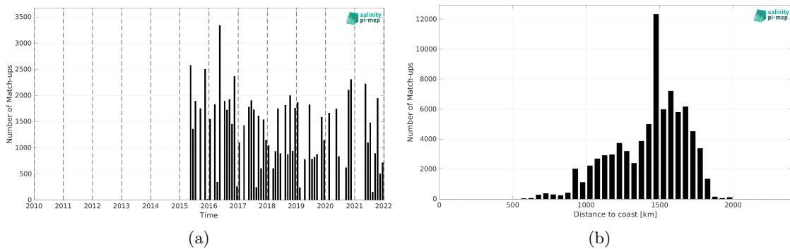
Figure 2: Number of match-ups between TSG (LEGOS-DM) and SMAP SSS L3 v5.3 - 8-Day running (RSS) SSS as a function of time (a) and as function of the distance to coast (b) over the SPURS 1 Pi-MEP region and for the full satellite product period.
