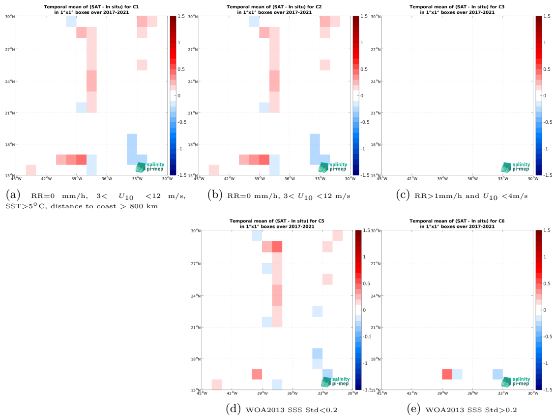
Figure 14: Temporal mean gridded over spatial boxes of size 1^\circ \times 1^\circ of \Delta SSS (SMAP SSS L3 v5.3 - 8-Day running (RSS) - TSG (GOSUD-Sailing-ship)) for 5 different subdatasets corresponding to:RR=0 mm/h, 3 < U_{10} < 12 m/s, SST >5^\circ C, distance to coast > 800 km (a), RR=0 mm/h, 3 < U_{10} < 12 m/s (b), RR >1 mm/h and U_{10} < 4 m/s (c), WOA2013 SSS Std <0.2 (d), WOA2013 SSS Std >0.2 (e).
