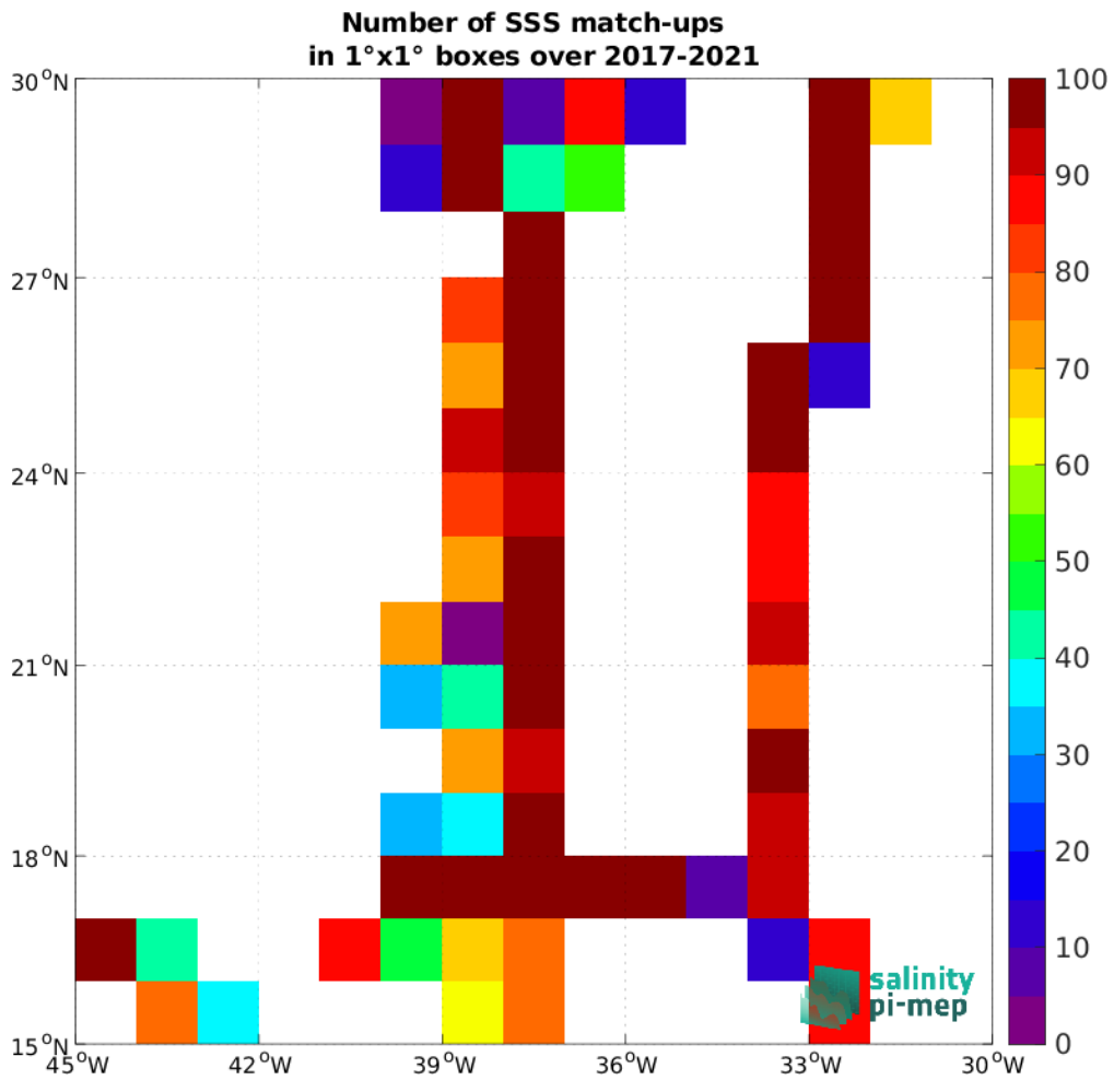
Figure 5: Number of SSS match-ups between TSG (GOSUD-Sailing-ship) SSS and the SMAP SSS L3 v5.3 - 8-Day running (RSS) SSS product for the SPURS 1 Pi-MEP region over 1^\circ \times 1^\circ boxes and for the full satellite product period.
