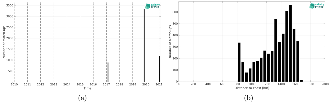
Figure 2: Number of match-ups between TSG (GOSUD-Sailing-ship) and SMAP SSS L3 v5.3 - 8-Day running (RSS) SSS as a function of time (a) and as function of the distance to coast (b) over the SPURS 1 Pi-MEP region and for the full satellite product period.
