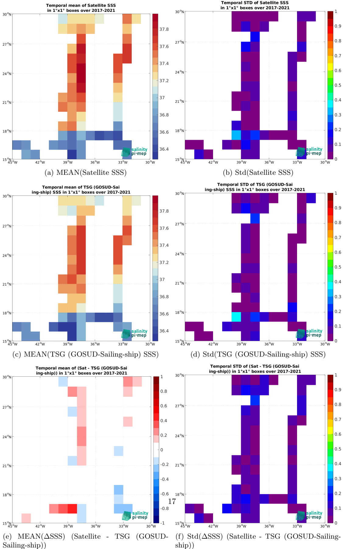
Figure 7: Temporal mean (left) and Std (right) of SSS from SMAP SSS L3 v5.3 - 8-Day running (RSS) (top), TSG (GOSUD-Sailing-ship) (middle), and of \Delta SSS (Satellite - TSG (GOSUD-Sailing-ship)). Only match-up pairs are used to generate these maps.
