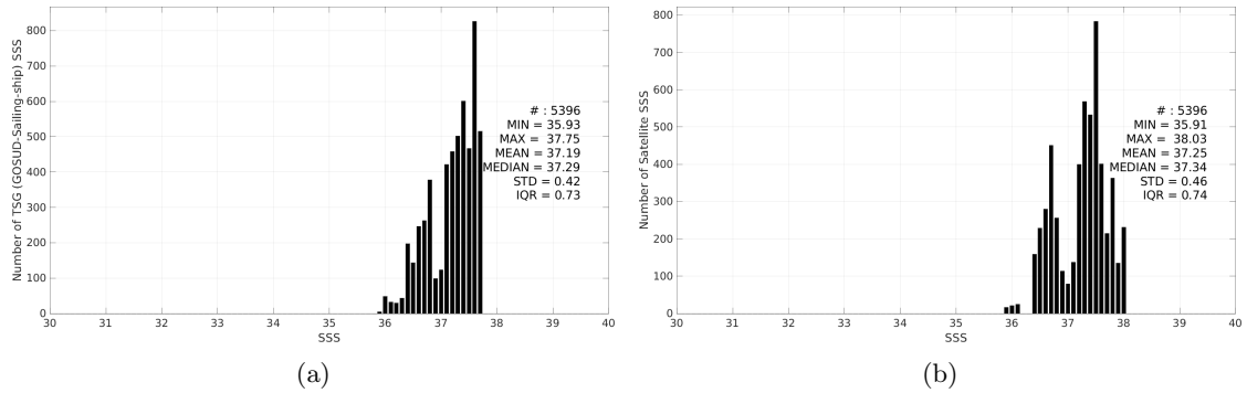
Figure 3: Histograms of SSS from TSG (GOSUD-Sailing-ship) (a) and SMAP SSS L3 v5.3 - 8-Day running (RSS) (b) considering all match-up pairs per bins of 0.1 over the SPURS 1 Pi-MEP region and for the full satellite product period.
