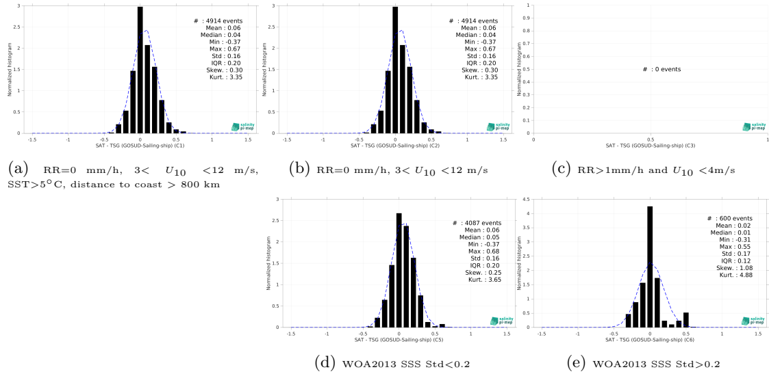
Figure 15: Normalized histogram of \Delta\text{SSS} (SMAP SSS L3 v5.3 - 8-Day running (RSS) - TSG (GOSUD-Sailing-ship)) for 5 different subdatasets corresponding to: RR=0 mm/h, 3 < U_{10} < 12 m/s, SST >5^{\circ}\text{C} , distance to coast > 800 km (a), RR=0 mm/h, 3 < U_{10} < 12 m/s (b), RR >1 mm/h and U_{10} < 4 m/s (c), WOA2013 SSS Std <0.2 (d), WOA2013 SSS Std >0.2 (e).
