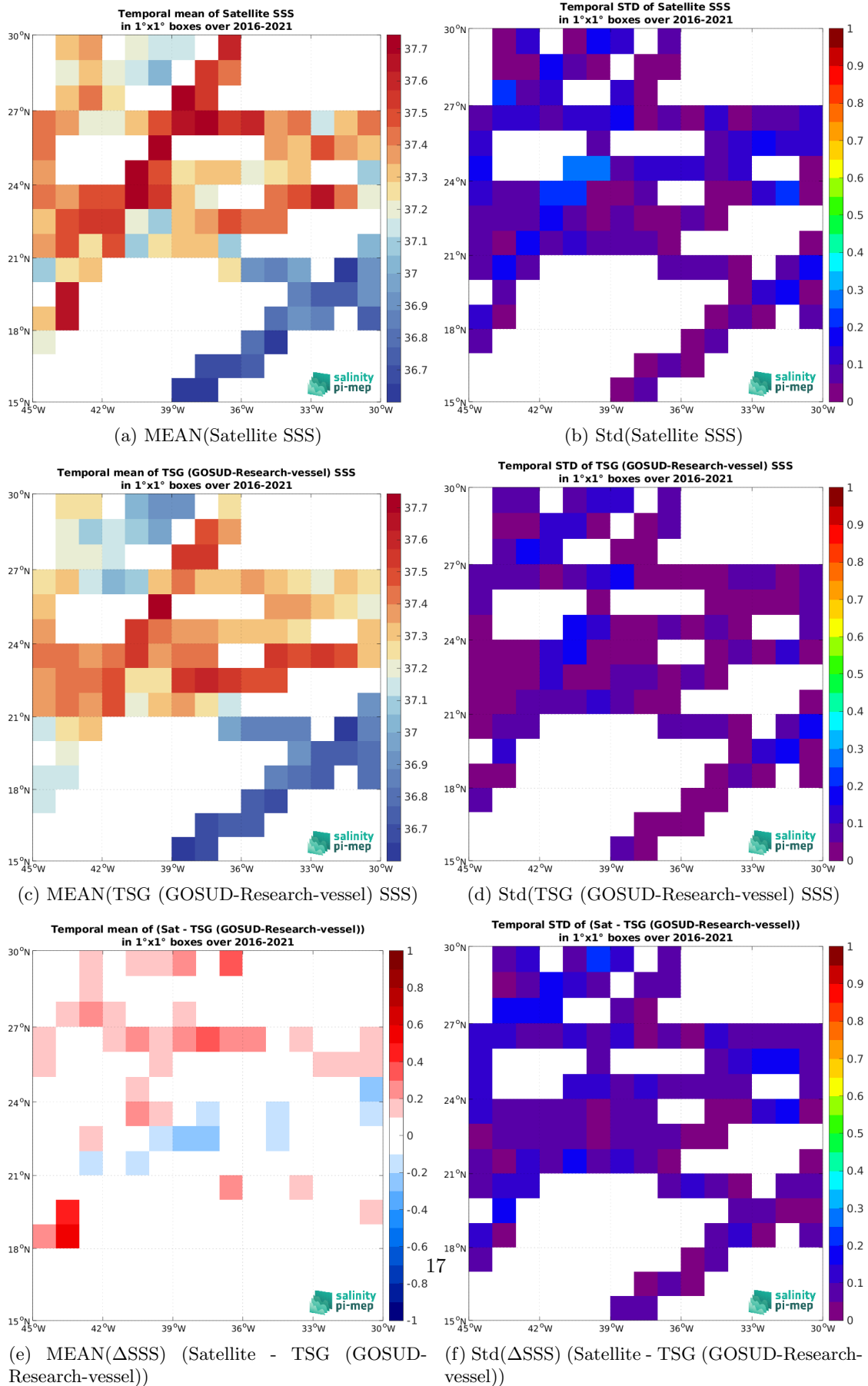
Figure 7: Temporal mean (left) and Std (right) of SSS from SMAP SSS L3 v5.3 - 8-Day running (RSS) (top), TSG (GOSUD-Research-vessel) (middle), and of \Delta SSS (Satellite - TSG (GOSUD-Research-vessel)). Only match-up pairs are used to generate these maps.
