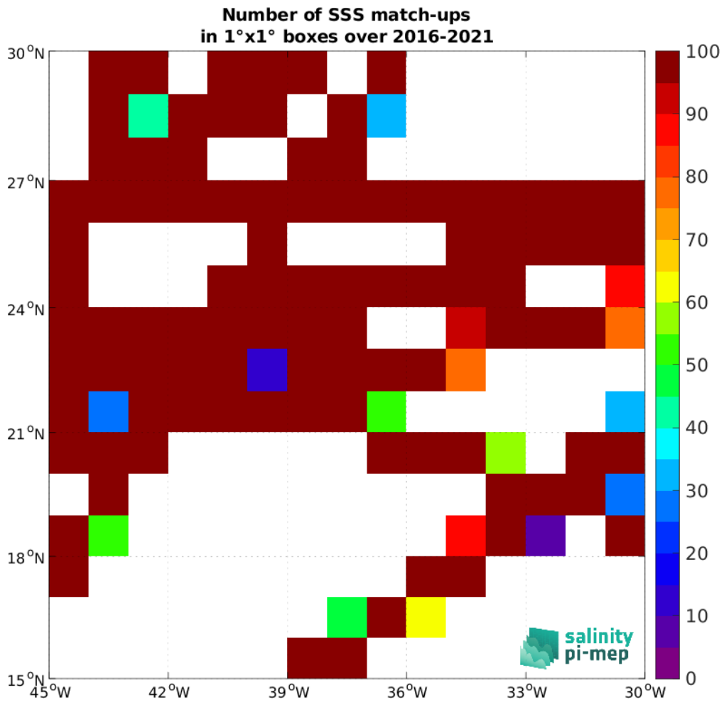
Figure 5: Number of SSS match-ups between TSG (GOSUD-Research-vessel) SSS and the SMAP SSS L3 v5.3 - 8-Day running (RSS) SSS product for the SPURS 1 Pi-MEP region over 1°x1° boxes and for the full satellite product period.
