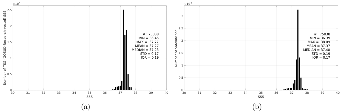
Figure 3: Histograms of SSS from TSG (GOSUD-Research-vessel) (a) and SMAP SSS L3 v5.3 - 8-Day running (RSS) (b) considering all match-up pairs per bins of 0.1 over the SPURS 1 Pi-MEP region and for the full satellite product period.
