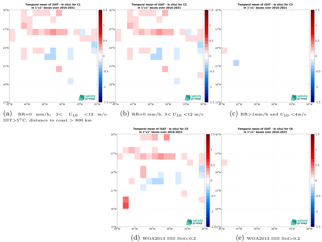
Figure 14: Temporal mean gridded over spatial boxes of size 1^\circ \times 1^\circ of \Delta SSS (SMAP SSS L3 v5.3 - 8-Day running (RSS) - TSG (GOSUD-Research-vessel)) for 5 different subdatasets corresponding to:RR=0 mm/h, 3 < U_{10} < 12 m/s, SST >5^\circ C, distance to coast > 800 km (a), RR=0 mm/h, 3 < U_{10} < 12 m/s (b), RR >1 mm/h and U_{10} < 4 m/s (c), WOA2013 SSS Std <0.2 (d), WOA2013 SSS Std >0.2 (e).
