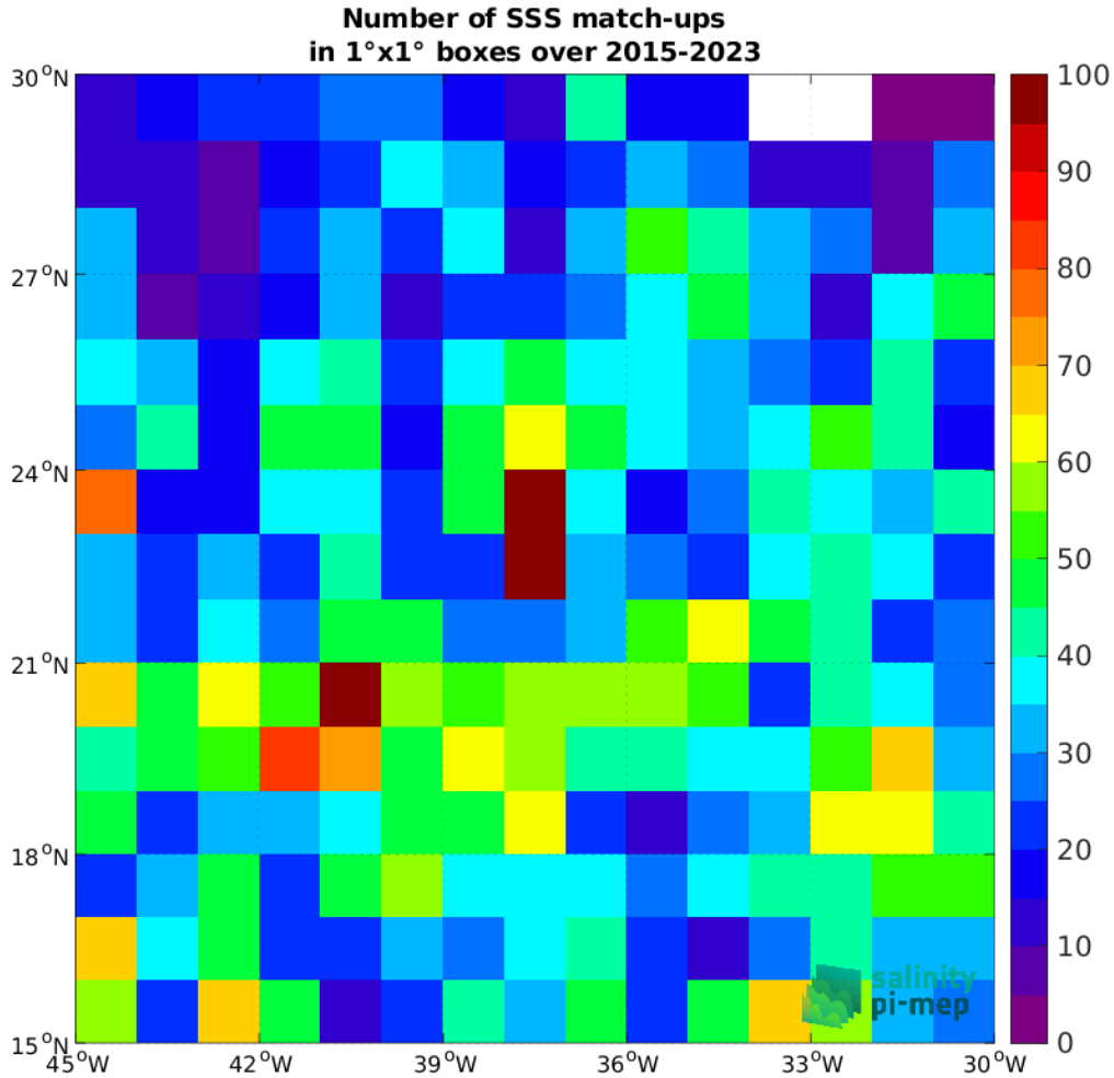
Figure 5: Number of SSS match-ups between Argo SSS and the SMAP SSS L3 v5.3 - 8-Day running (RSS) SSS product for the SPURS 1 Pi-MEP region over 1^\circ \times 1^\circ boxes and for the full satellite product period.
