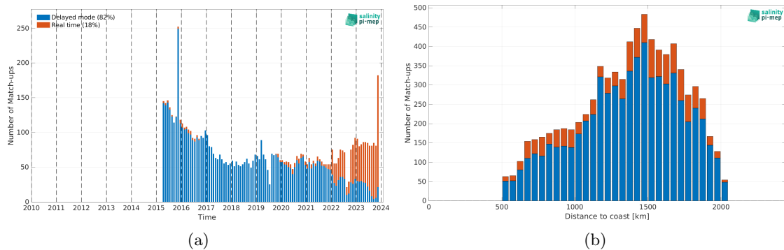
Figure 2: Number of match-ups between Argo and SMAP SSS L3 v5.3 - 8-Day running (RSS) SSS as a function of time (a) and as function of the distance to coast (b) over the SPURS 1 Pi-MEP region and for the full satellite product period.
