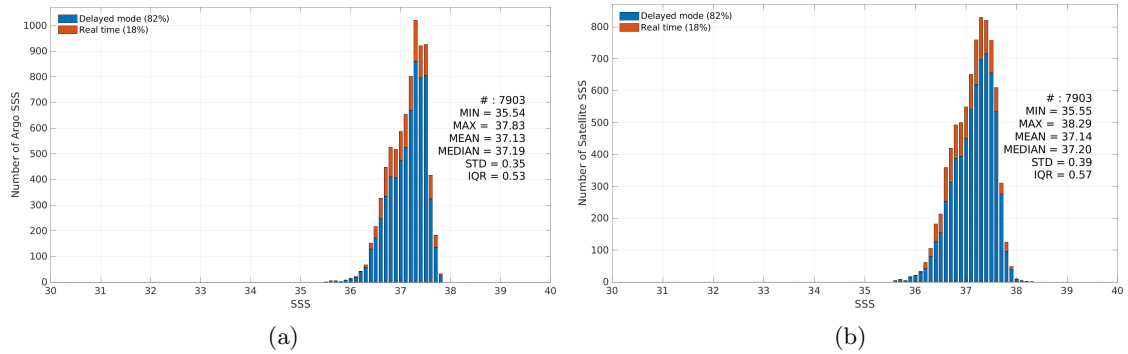
Figure 3: Histograms of SSS from Argo (a) and SMAP SSS L3 v5.3 - 8-Day running (RSS) (b) considering all match-up pairs per bins of 0.1 over the SPURS 1 Pi-MEP region and for the full satellite product period.
