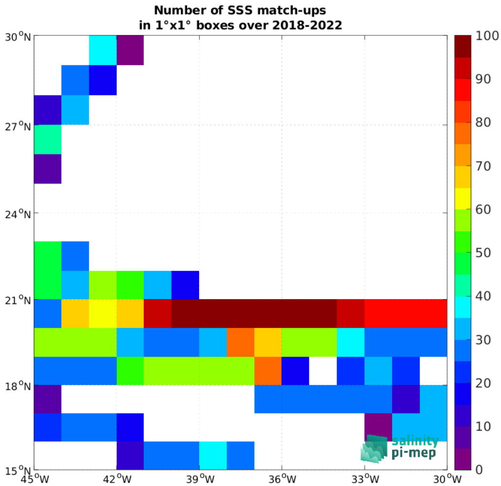
Figure 5: Number of SSS match-ups between TSG (SAMOS) SSS and the SMAP SSS L3 v5.3 - Monthly (RSS) SSS product for the SPURS 1 Pi-MEP region over 1^\circ \times 1^\circ boxes and for the full satellite product period.
