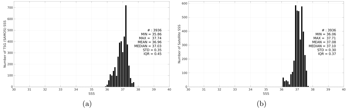
Figure 3: Histograms of SSS from TSG (SAMOS) (a) and SMAP SSS L3 v5.3 - Monthly (RSS) (b) considering all match-up pairs per bins of 0.1 over the SPURS 1 Pi-MEP region and for the full satellite product period.
