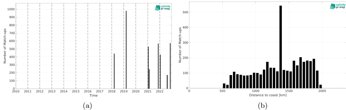
Figure 2: Number of match-ups between TSG (SAMOS) and SMAP SSS L3 v5.3 - Monthly (RSS) SSS as a function of time (a) and as function of the distance to coast (b) over the SPURS 1 Pi-MEP region and for the full satellite product period.
