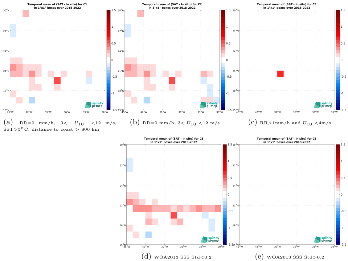
Figure 14: Temporal mean gridded over spatial boxes of size 1^\circ \times 1^\circ of \Delta\text{SSS} (SMAP SSS L3 v5.3 - Monthly (RSS) - TSG (SAMOS)) for 5 different subdatasets corresponding to: \text{RR}=0 \text{ mm/h} , 3 < U_{10} < 12 \text{ m/s} , \text{SST} > 5^\circ\text{C} , distance to coast > 800 \text{ km} (a), \text{RR}=0 \text{ mm/h} , 3 < U_{10} < 12 \text{ m/s} (b), \text{RR} > 1 \text{ mm/h} and U_{10} < 4 \text{ m/s} (c), WOA2013 SSS Std < 0.2 (d), WOA2013 SSS Std > 0.2 (e).
