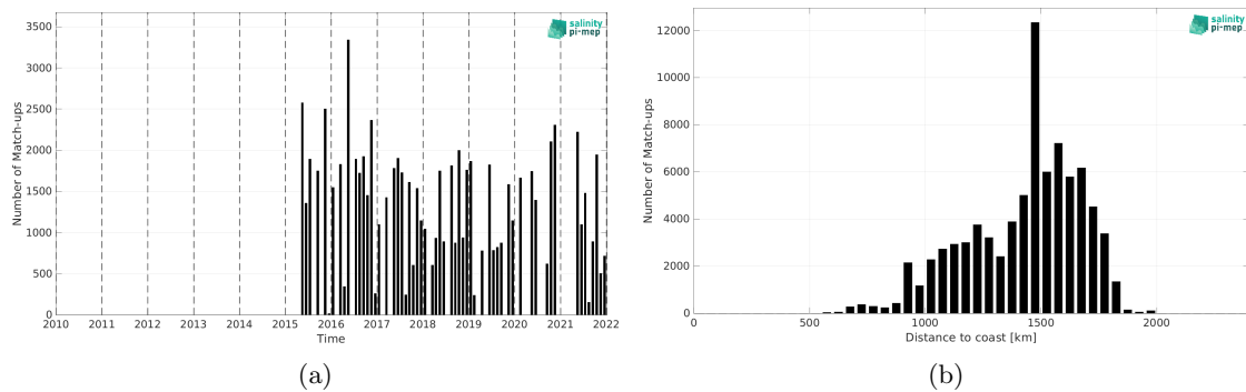
Figure 2: Number of match-ups between TSG (LEGOS-DM) and SMAP SSS L3 v5.3 - Monthly (RSS) SSS as a function of time (a) and as function of the distance to coast (b) over the SPURS 1 Pi-MEP region and for the full satellite product period.
