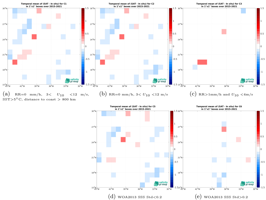
Figure 14: Temporal mean gridded over spatial boxes of size 1^\circ \times 1^\circ of \Delta SSS (SMAP SSS L3 v5.3 - Monthly (RSS) - TSG (LEGOS-DM)) for 5 different subdatasets corresponding to: RR=0 mm/h, 3 < U_{10} < 12 m/s, SST > 5^\circ C , distance to coast > 800 km (a), RR=0 mm/h, 3 < U_{10} < 12 m/s (b), RR > 1 mm/h and U_{10} < 4 m/s (c), WOA2013 SSS Std < 0.2 (d), WOA2013 SSS Std > 0.2 (e).
