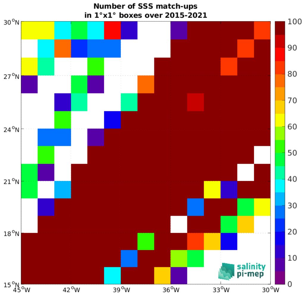
Figure 5: Number of SSS match-ups between TSG (LEGOS-DM) SSS and the SMAP SSS L3 v5.3 - Monthly (RSS) SSS product for the SPURS 1 Pi-MEP region over 1°x1° boxes and for the full satellite product period.
