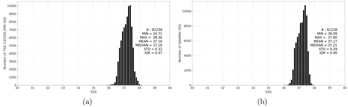
Figure 3: Histograms of SSS from TSG (LEGOS-DM) (a) and SMAP SSS L3 v5.3 - Monthly (RSS) (b) considering all match-up pairs per bins of 0.1 over the SPURS 1 Pi-MEP region and for the full satellite product period.
