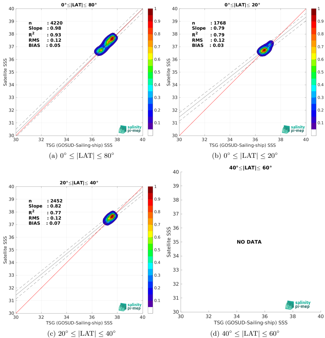
Figure 10: Contour maps of the concentration of SMAP SSS L3 v5.3 - Monthly (RSS) SSS (y-axis) versus TSG (GOSUD-Sailing-ship) SSS (x-axis) at match-up pairs for different latitude bands. For each plot, the red line shows x=y . The black thin and dashed lines indicate a linear fit through the data cloud and the \pm 95\% confidence levels, respectively. The number match-up pairs n , the slope and R^2 coefficient of the linear fit, the root mean square (RMS) and the mean bias between satellite and in situ data are indicated for each latitude band in each plots.
