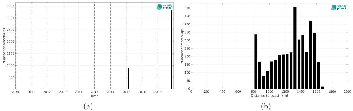
Figure 2: Number of match-ups between TSG (GOSUD-Sailing-ship) and SMAP SSS L3 v5.3 - Monthly (RSS) SSS as a function of time (a) and as function of the distance to coast (b) over the SPURS 1 Pi-MEP region and for the full satellite product period.
