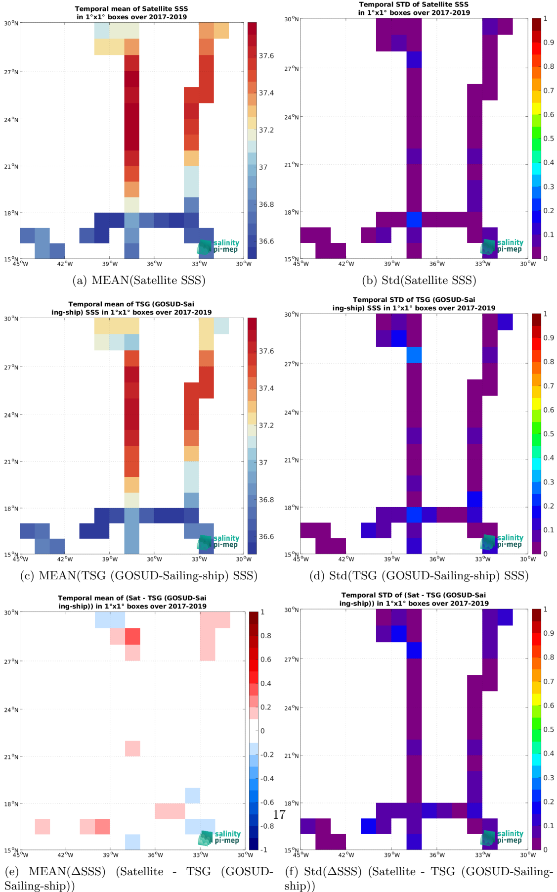
Figure 7: Temporal mean (left) and Std (right) of SSS from SMAP SSS L3 v5.3 - Monthly (RSS) (top), TSG (GOSUD-Sailing-ship) (middle), and of \Delta SSS (Satellite - TSG (GOSUD-Sailing-ship)). Only match-up pairs are used to generate these maps.
