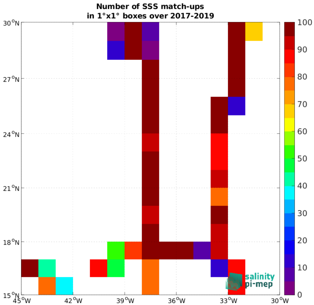
Figure 5: Number of SSS match-ups between TSG (GOSUD-Sailing-ship) SSS and the SMAP SSS L3 v5.3 - Monthly (RSS) SSS product for the SPURS 1 Pi-MEP region over 1°x1° boxes and for the full satellite product period.
