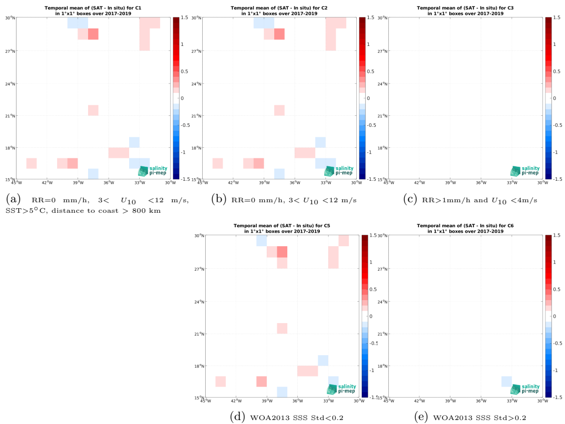
Figure 14: Temporal mean gridded over spatial boxes of size 1^\circ \times 1^\circ of \Delta\text{SSS} (SMAP SSS L3 v5.3 - Monthly (RSS) - TSG (GOSUD-Sailing-ship)) for 5 different subdatasets corresponding to: \text{RR}=0 \text{ mm/h} , 3 < U_{10} < 12 \text{ m/s} , \text{SST} > 5^\circ\text{C} , distance to coast > 800 \text{ km} (a), \text{RR}=0 \text{ mm/h} , 3 < U_{10} < 12 \text{ m/s} (b), \text{RR} > 1\text{mm/h} and U_{10} < 4\text{m/s} (c), WOA2013 SSS Std < 0.2 (d), WOA2013 SSS Std > 0.2 (e).
