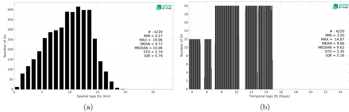
Figure 6: Histograms of the spatial (a) and temporal (b) lags between the location/time of the TSG (GOSUD-Sailing-ship) measurement and the date of the corresponding SMAP SSS L3 v5.3 - Monthly (RSS) SSS pixel.
