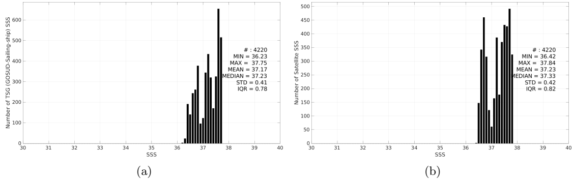
Figure 3: Histograms of SSS from TSG (GOSUD-Sailing-ship) (a) and SMAP SSS L3 v5.3 - Monthly (RSS) (b) considering all match-up pairs per bins of 0.1 over the SPURS 1 Pi-MEP region and for the full satellite product period.
