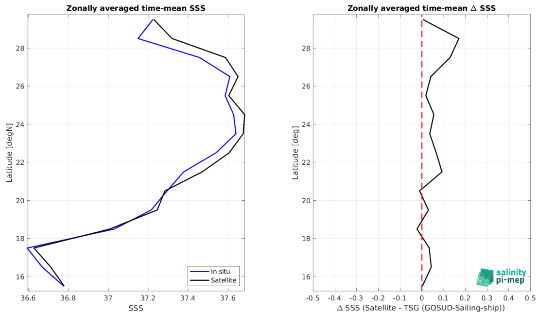
Figure 9: Left panel: Zonal mean SSS from SMAP SSS L3 v5.3 - Monthly (RSS) satellite product (black) and from TSG (GOSUD-Sailing-ship) (blue). Right panel: Zonal mean of \Delta SSS (Satellite - TSG (GOSUD-Sailing-ship)) for all the collected Pi-MEP match-up pairs estimated over the full satellite product period.
