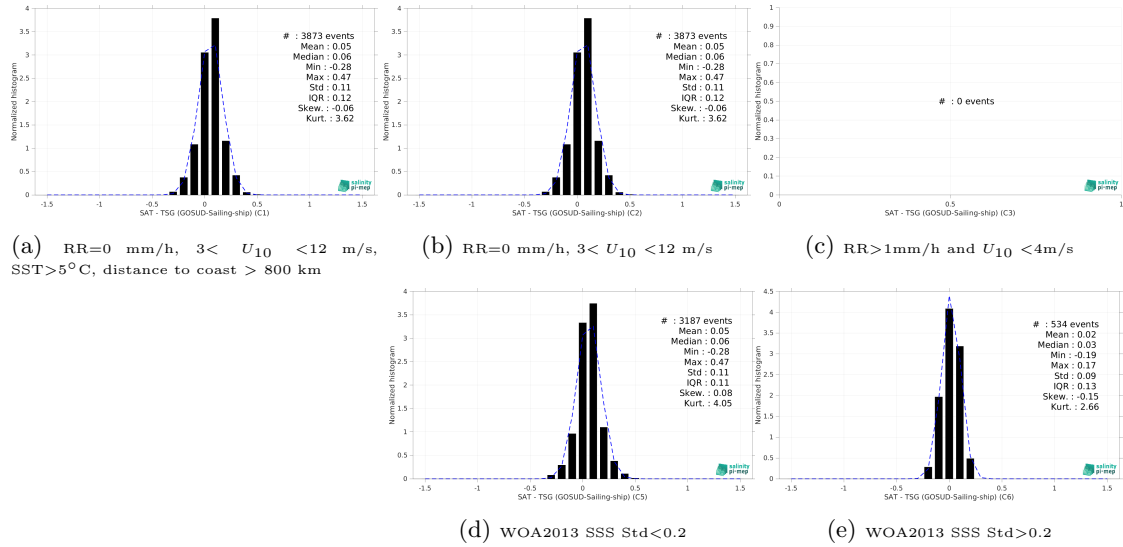
Figure 15: Normalized histogram of \Delta SSS (SMAP SSS L3 v5.3 - Monthly (RSS) - TSG (GOSUD-Sailing-ship)) for 5 different subdatasets corresponding to: RR=0 mm/h, 3 < U_{10} < 12 m/s, SST > 5°C, distance to coast > 800 km (a), RR=0 mm/h, 3 < U_{10} < 12 m/s (b), RR > 1mm/h and U_{10} < 4 m/s (c), WOA2013 SSS Std < 0.2 (d), WOA2013 SSS Std > 0.2 (e).
