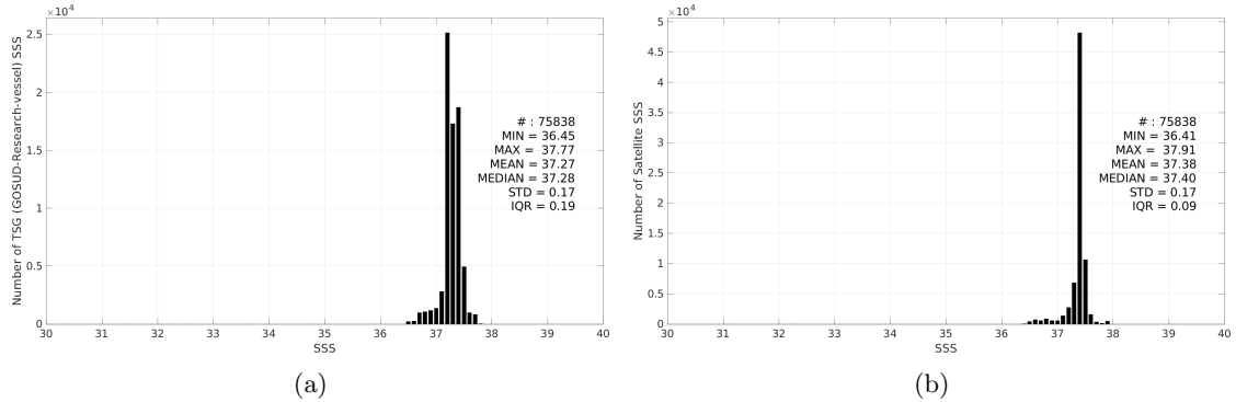
Figure 3: Histograms of SSS from TSG (GOSUD-Research-vessel) (a) and SMAP SSS L3 v5.3 - Monthly (RSS) (b) considering all match-up pairs per bins of 0.1 over the SPURS 1 Pi-MEP region and for the full satellite product period.
