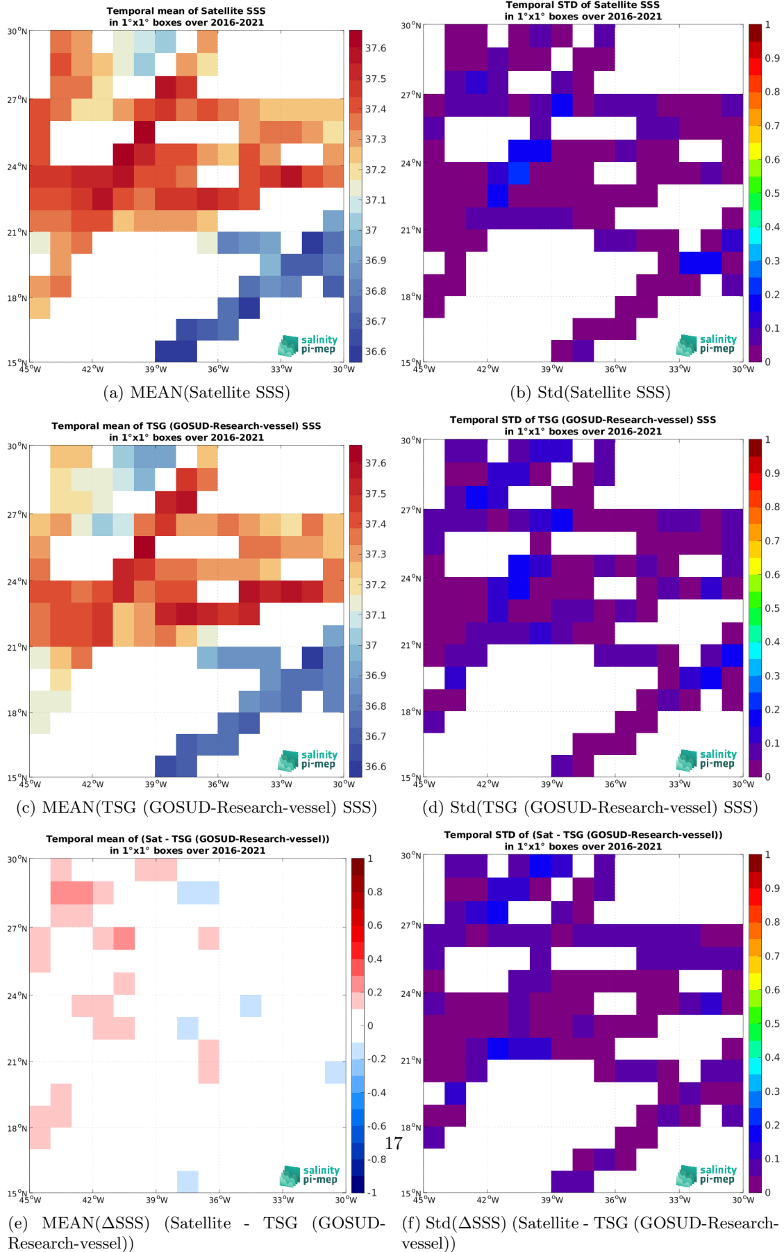
Figure 7: Temporal mean (left) and Std (right) of SSS from SMAP SSS L3 v5.3 - Monthly (RSS) (top), TSG (GOSUD-Research-vessel) (middle), and of \Delta SSS (Satellite - TSG (GOSUD-Research-vessel)). Only match-up pairs are used to generate these maps.
