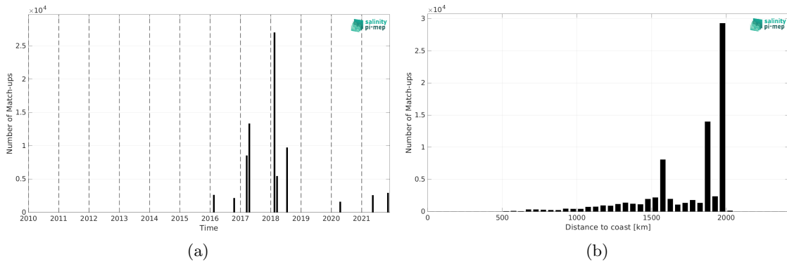
Figure 2: Number of match-ups between TSG (GOSUD-Research-vessel) and SMAP SSS L3 v5.3 - Monthly (RSS) SSS as a function of time (a) and as function of the distance to coast (b) over the SPURS 1 Pi-MEP region and for the full satellite product period.
