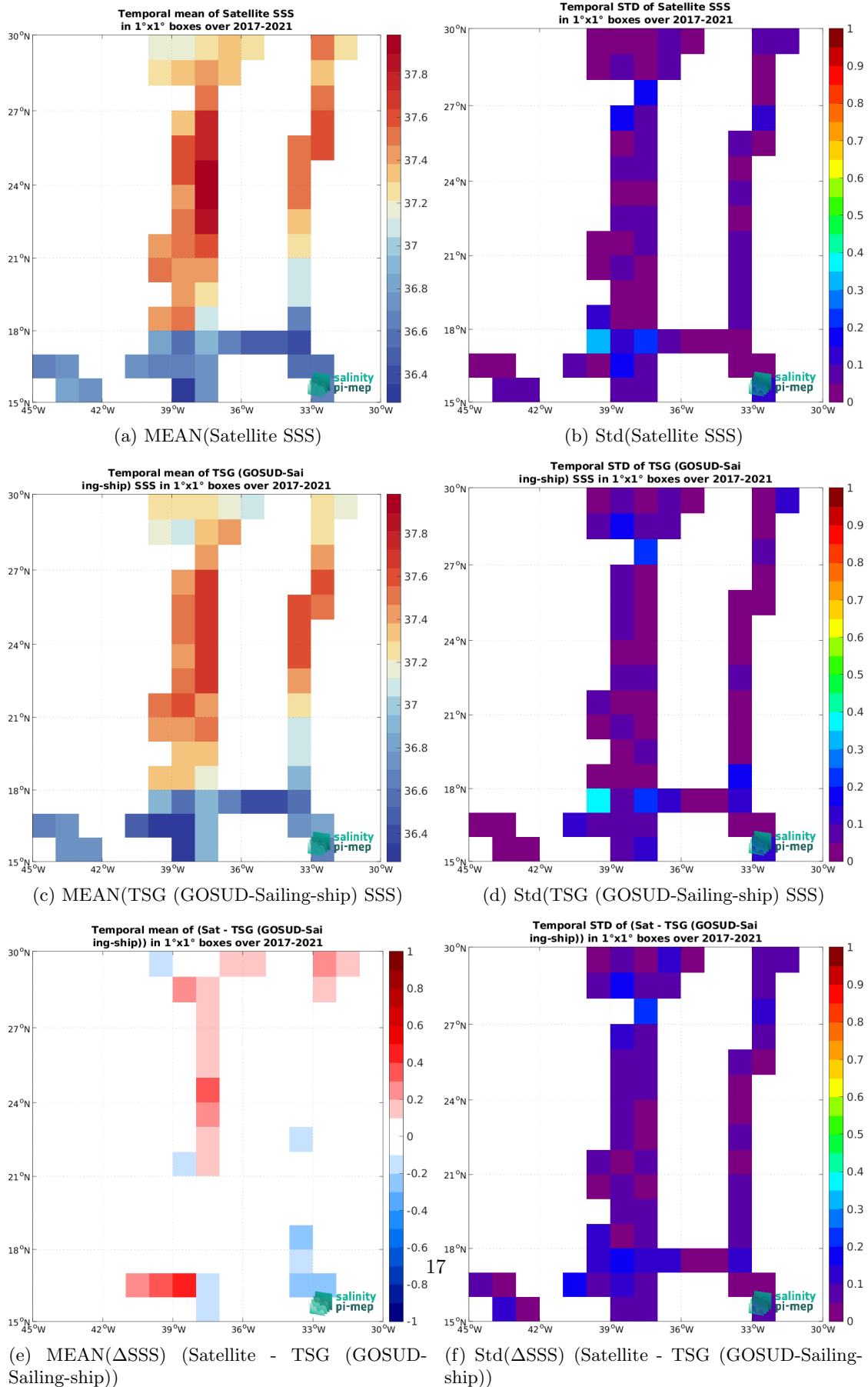
Figure 6: Temporal mean (left) and Std (right) of SSS from SMAP SSS L3 v5 - 8-Day running (RSS) (top), TSG (GOSUD-Sailing-ship) (middle), and of \Delta SSS (Satellite - TSG (GOSUD-Sailing-ship)). Only match-up pairs are used to generate these maps.
