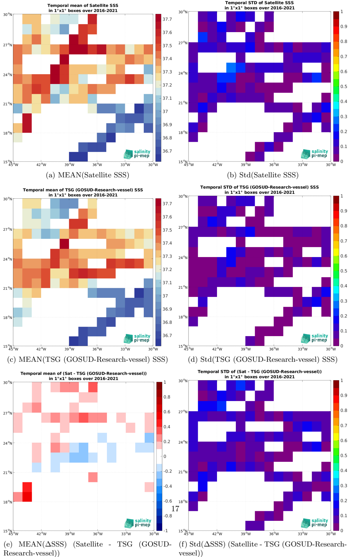
Figure 6: Temporal mean (left) and Std (right) of SSS from SMAP SSS L3 v5 - 8-Day running (RSS) (top), TSG (GOSUD-Research-vessel) (middle), and of \Delta SSS (Satellite - TSG (GOSUD-Research-vessel)). Only match-up pairs are used to generate these maps.
