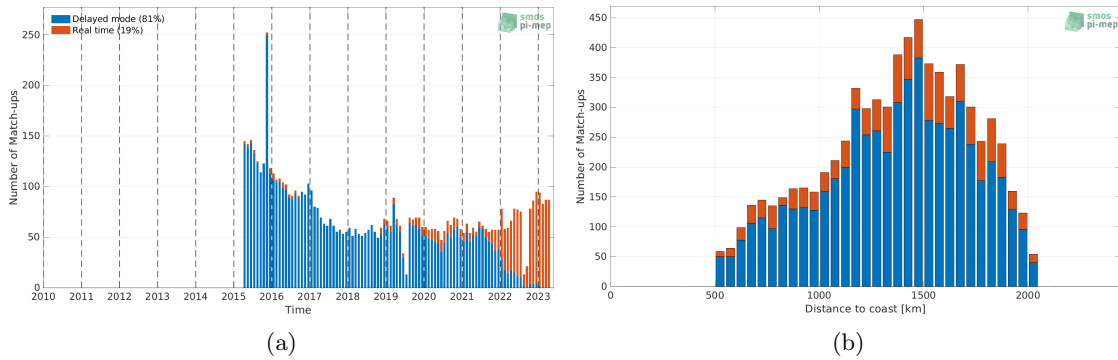
Figure 1: Number of match-ups between Argo and SMAP SSS L3 v5 - 8-Day running (RSS) SSS as a function of time (a) and as function of the distance to coast (b) over the SPURS 1 Pi-MEP region and for the full satellite product period.
