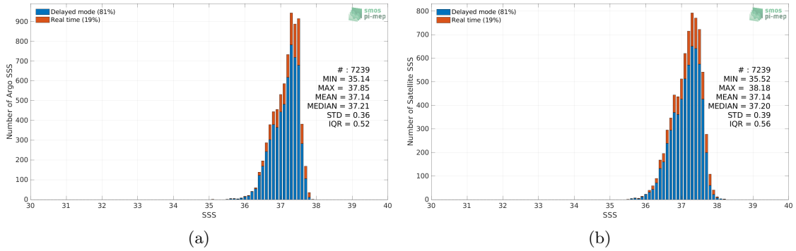
Figure 2: Histograms of SSS from Argo (a) and SMAP SSS L3 v5 - 8-Day running (RSS) (b) considering all match-up pairs per bins of 0.1 over the SPURS 1 Pi-MEP region and for the full satellite product period.
