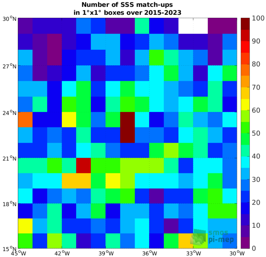
Figure 4: Number of SSS match-ups between Argo SSS and the SMAP SSS L3 v5 - 8-Day running (RSS) SSS product for the SPURS 1 Pi-MEP region over 1°x1° boxes and for the full satellite product period.
