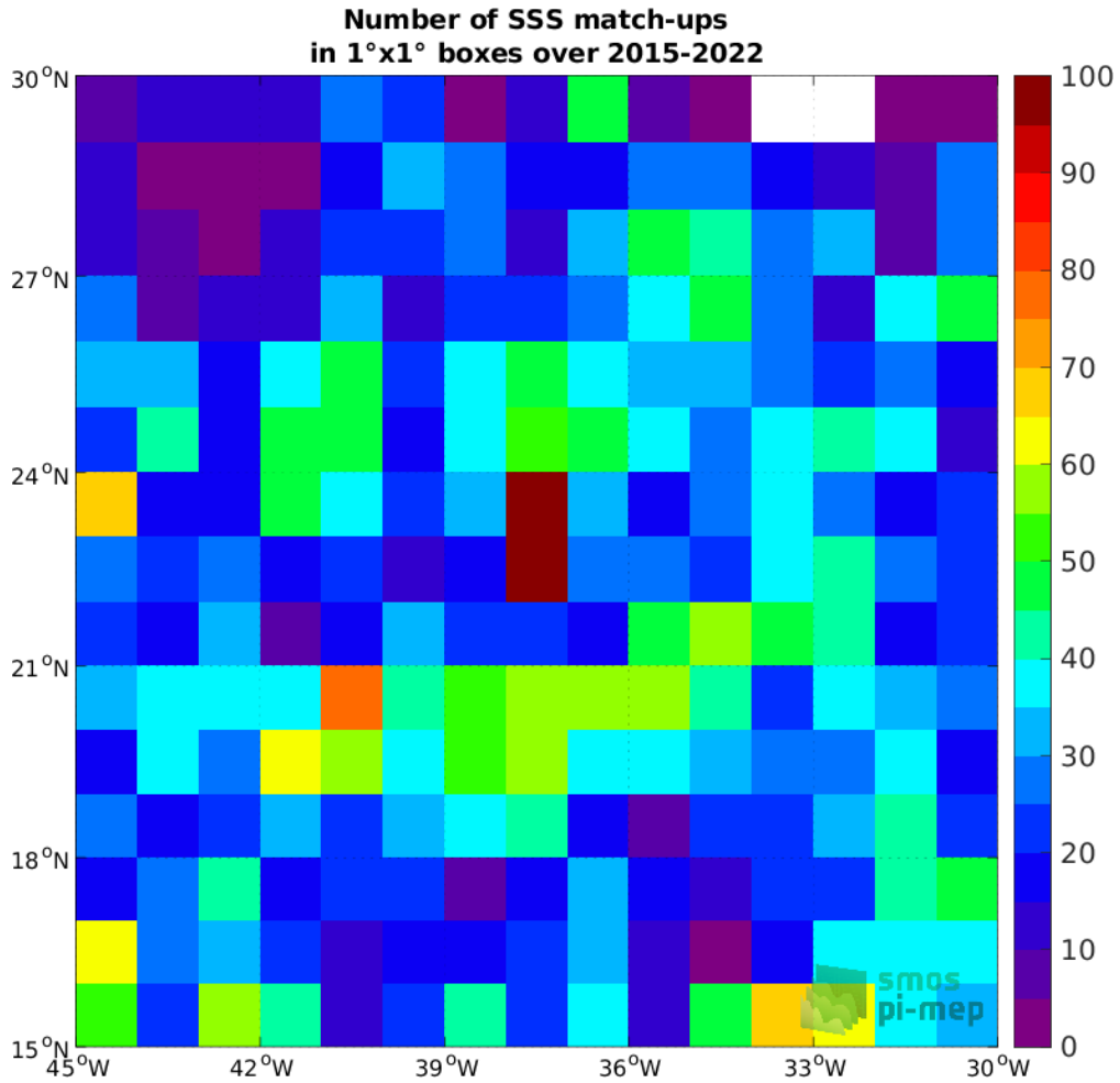
Figure 4: Number of SSS match-ups between Argo SSS and the SMAP SSS L3 v5 - 8-Day running (RSS) SSS product for the SPURS 1 Pi-MEP region over 1^\circ \times 1^\circ boxes and for the full satellite product period.
